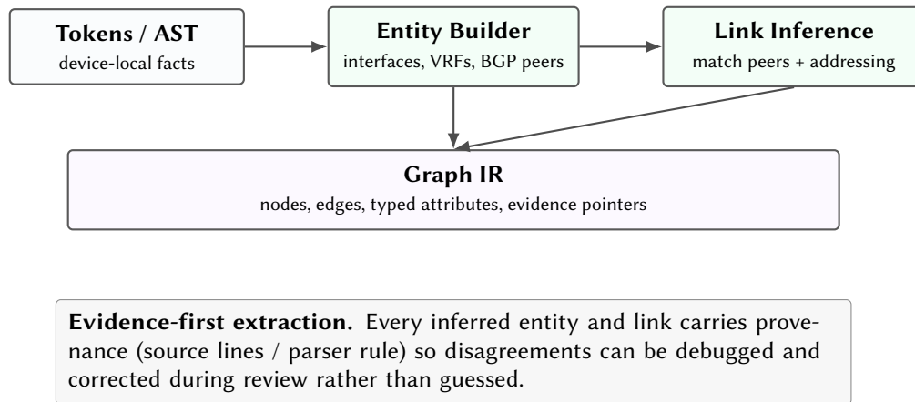
Figure 2. Topology extraction as a graph construction problem: facts are lifted into entities, then joined into links with explicit provenance.
