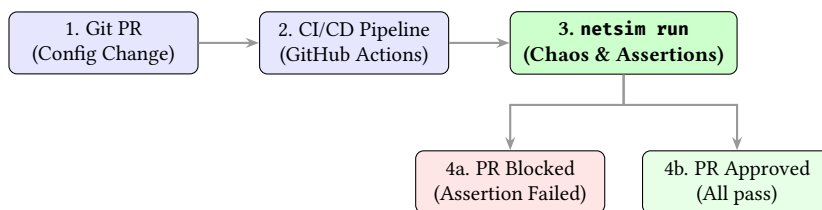
Figure 9. CI/CD Pipeline Integration. Declarative assertions allow netsim to automatically block PRs that would introduce routing loops or isolation, preventing operator-induced outages before deployment.
