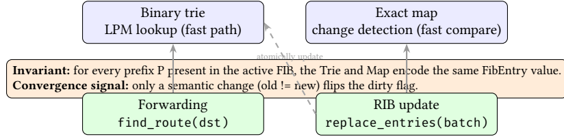
Figure 5. Dual-Index FIB as an Invariant. The trie serves the forwarding fast path (LPM), while the exact-map enables constant-time equality checks during updates so convergence is reset only on real semantic changes. Both indices are updated atomically to preserve coherence.
