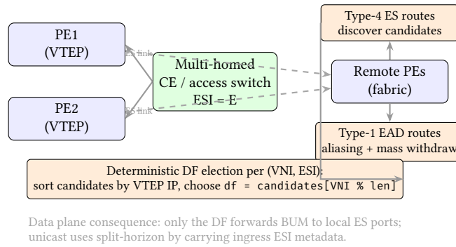
Figure 13. EVPN Multi-Homing as Deterministic Control/Data Coupling. Type-4 routes discover the candidate set for an Ethernet Segment (ESI). A deterministic DF election per VNI selects which PE forwards BUM to local ES ports, while split-horizon prevents loops by dropping frames that would hairpin back onto the same ESI.
