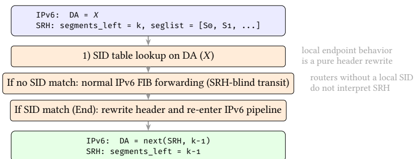
Figure 8. SRv6 Packet Walk as a Header-Rewrite Semantics. A local SID match triggers endpoint behavior that deterministically rewrites (DA, segments_left) and loops back into the IPv6 forwarding pipeline. Routers without a matching local SID forward on the outer DA only.
