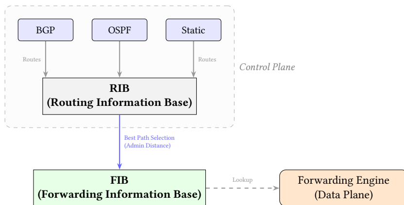
Figure 4. RIB/FIB Separation. Multiple routing protocols populate the global RIB. The router executes best-path selection based on Administrative Distance to program the active FIB used by the forwarding engine.
