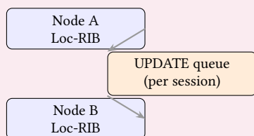
Figure 12. EVPN Synchronisation as a Consistency Model. Per-message queuing exposes the simulation to ordering-dependent behaviour. netsim instead snapshots all EVPN Loc-RIBs once per tick (Phase P2.5) and applies the same snapshot everywhere, providing a deterministic barrier that preserves “simultaneous” control-plane state replication.
