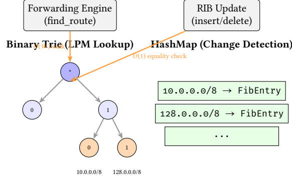
Figure 6. Dual-Index FIB Architecture. The Forwarding Engine uses the Binary Trie for fast Longest-Prefix-Match lookups, while RIB updates use the HashMap for O(1) exact-match change detection to avoid spurious convergence resets.
