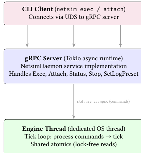
Figure 14. Daemon Concurrency Architecture. A Tokio-based gRPC server receives concurrent client connections and forwards commands to the strictly single-threaded Engine via channels.
