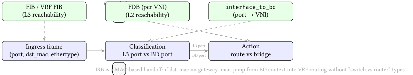
Figure 11. Unified L2/L3 Router as a Conceptual Model. Rather than branching on device type, the data plane classifies each ingress by port-to-bridge-domain membership and then selects an action (route via FIB/VRF or bridge via per-VNI FDB). IRB is a deterministic MAC-based handoff from L2 to L3.
