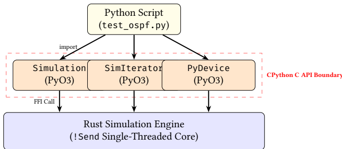
Figure 15. Python Bindings Architecture. The PyO3 wrappers expose the single-threaded Rust Engine directly to the Python interpreter, allowing zero-copy, in-process access to the simulation state.
