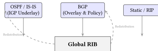
Figure 7. Control Plane Protocol Interactions. Protocols independently compute routes and submit them to the Global RIB, which arbitrates conflicts using administrative distance. The RIB can also redistribute routes back into protocols.
