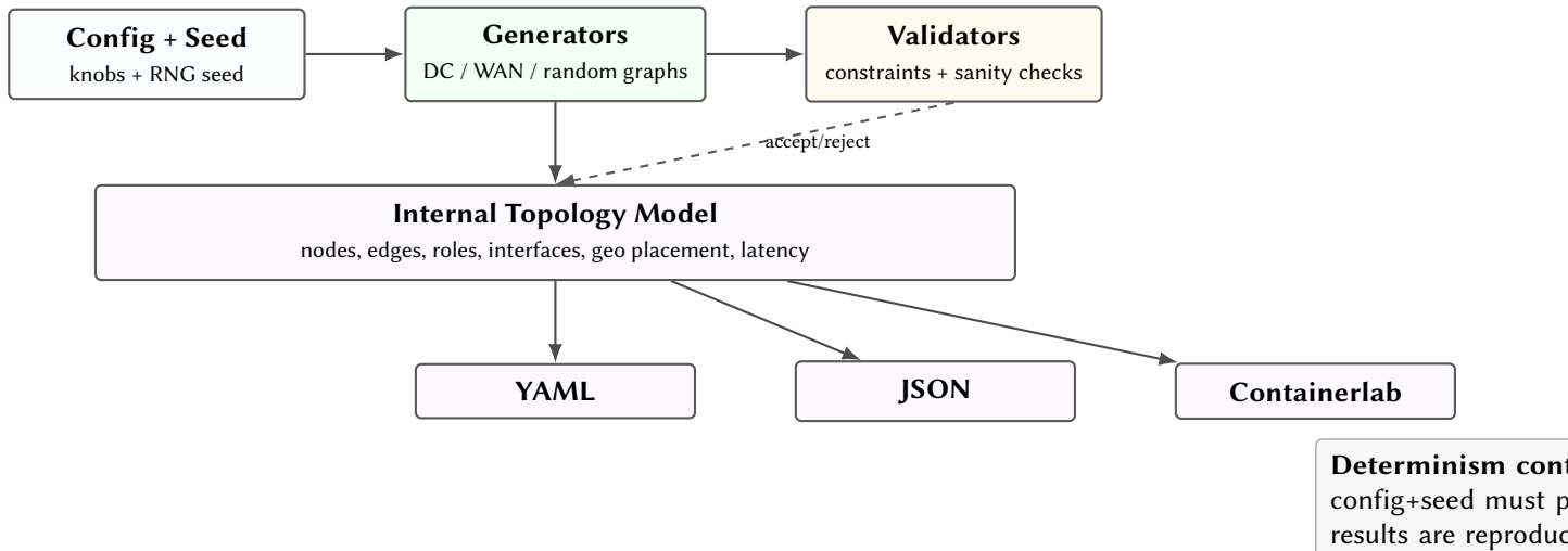
Figure 1. TopoGen end-to-end architecture: seeded generation into a typed internal model, followed by validation and export.
