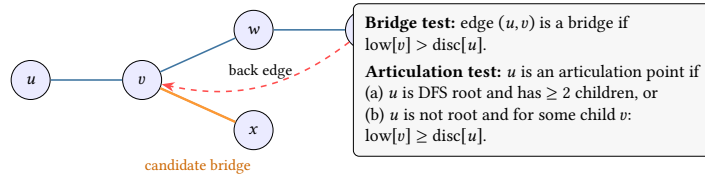
Figure 23. Tarjan-style SPOF primitives. Discovery times ( \text{disc} ) order the DFS tree; low-link values ( \text{low} ) summarise whether a subtree has a back-edge escape route. The bridge/articulation tests are simple comparisons once \text{low} is known.
