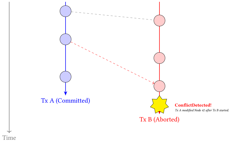
Figure 42. MVCC Transaction Timeline. Both transactions read from the same initial snapshot S_0 . Because Tx A commits a mutation to Node 42 before Tx B attempts to mutate it, the Conflict Engine safely aborts Tx B to prevent a Write-Write conflict.
