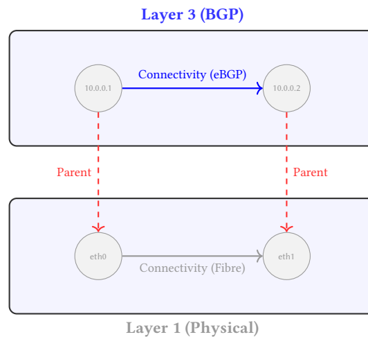
Figure 9. Cross-Layer Relationships. L3 BGP Endpoints are bound to L1 Physical Endpoints via Parent edges. If eth0 fails, the engine traverses the incoming Parent edge to deterministically tear down the dependent BGP session.
