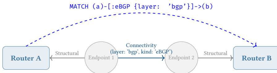
Figure 33. Virtual Cypher Translation. The user specifies a semantic device-to-device relationship (dashed line). The query planner intercepts this and automatically compiles it into the three-hop endpoint traversal (solid lines) required by the structural data model.
