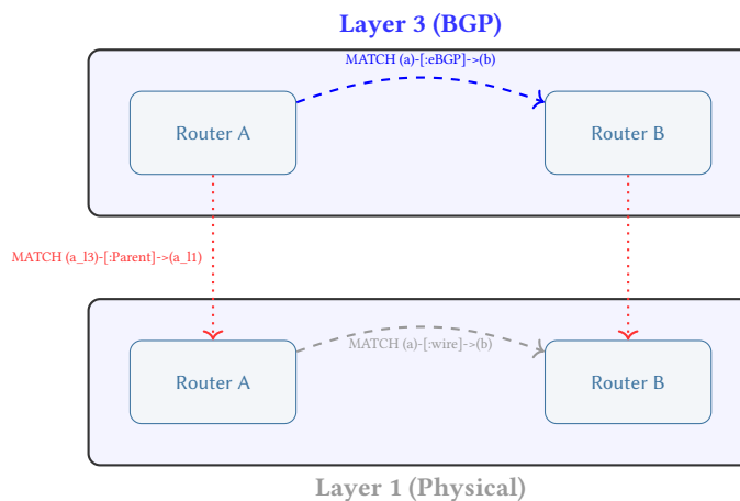
Figure 35. Cross-Layer Semantic Querying. Users can independently query the semantic graph of each layer and trace dependencies across them using the Parent edges, entirely abstracted from the underlying port complexities.
