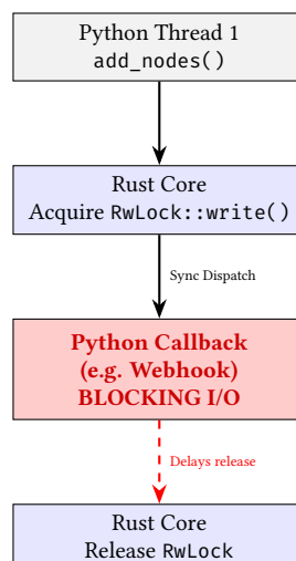
Figure 51. The Event Callback Danger Zone. Synchronous callbacks hold the engine's global write lock. Future versions will move to a lock-free async queue design.
