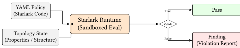
Figure 13. Starlark Policy Evaluation. The sandboxed runtime safely evaluates Python-like policy code against the topology state to generate deterministic compliance findings.
