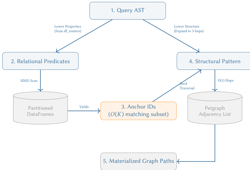
Figure 36. The Filter-First Hybrid Execution Pipeline. During the AST compilation phase, the engine splits the query. It executes highly-selective property predicates against partitioned columnar storage first , yielding a tiny subset of Anchor IDs. These anchors seed the expanded 3-hop structural graph traversal, guaranteeing that the engine never traces paths from irrelevant nodes.
