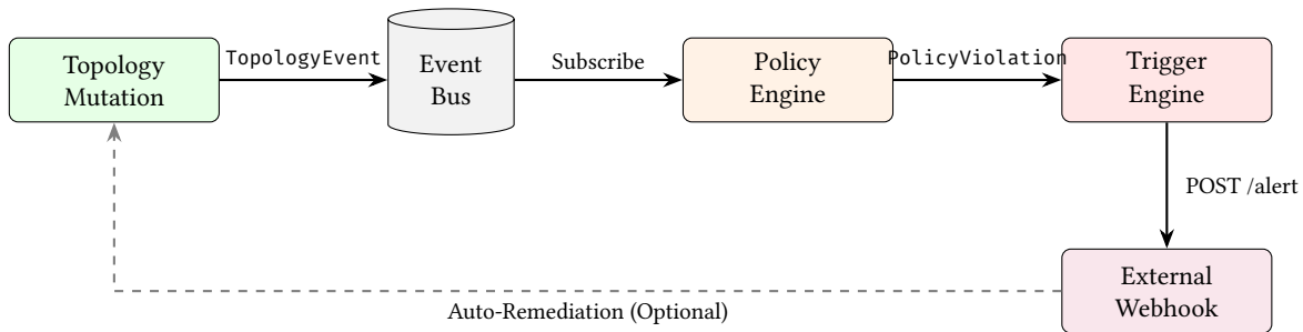
Figure 59. Proposed Reactive Topology workflow: Automated policy validation pushing events to the Trigger Engine rather than waiting for pull-based queries.
