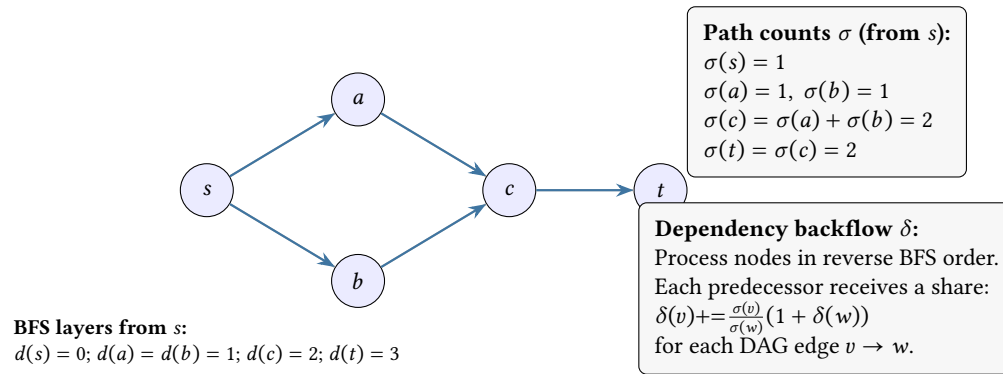
Figure 18. Brandes betweenness centrality as a conserved “flow” on the shortest-path DAG. The forward BFS counts how many shortest paths reach each node ( \sigma ). The reverse accumulation distributes dependency ( \delta ) back to predecessors in proportion to their contribution.
