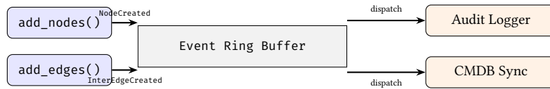
Figure 52. The Reactive Event Pipeline. Mutations in the core engine generate events which are buffered and asynchronously dispatched to Python callbacks.
