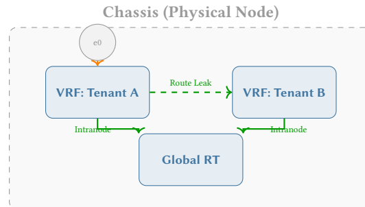
Figure 7. Intranode edges within a chassis. VRF sub-nodes connect to the Global Routing Table via Intranode edges. Each sub-node can optionally own its own Endpoints (shown on VRF: Tenant A). The dashed edge represents a route-leak relationship.
