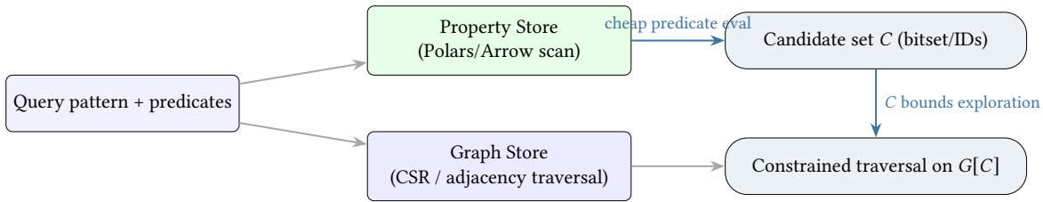
Figure 20. Filter-first planning as candidate-set narrowing. Property predicates are evaluated first to produce a set C of eligible nodes/edges. Structural traversal then runs against the induced subgraph G[C] , avoiding work on irrelevant regions of the topology.
