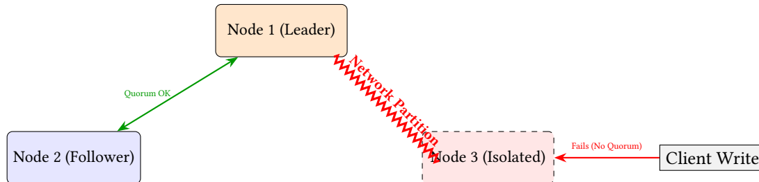
Figure 56. Split-Brain Resolution. In a partition, the isolated Node 3 rejects writes because it cannot replicate logs to a majority quorum. Nodes 1 and 2 continue processing safely.
