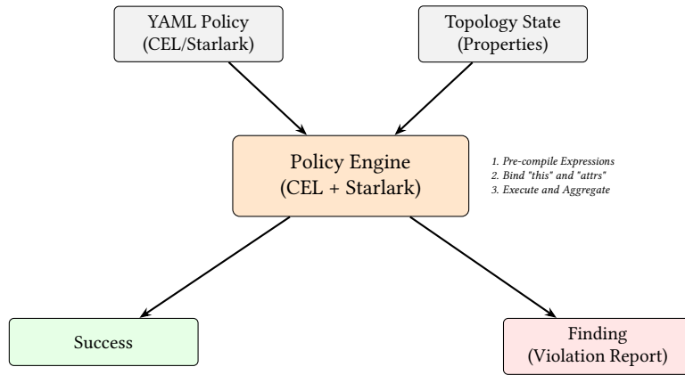
Figure 14. Policy Evaluation Pipeline. The engine pre-compiles declarative CEL expressions and procedural Starlark logic, executing them against a unified topology context to generate structured findings.
