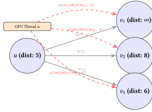
Figure 48. GPU SSSP relaxation. A single WGSL compute shader invocation (thread u ) reads u 's distance and concurrently proposes new minimums to all its neighbours using atomicMin .
