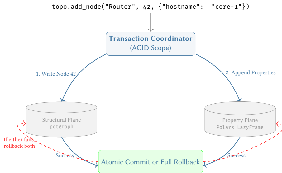
Figure 41. The Dual-Write Transaction Model. Mutations are coordinated atomically across the divergent storage engines. If a node is added to the graph but the properties fail schema validation in Polars, the entire transaction aborts, ensuring the digital twin never enters a split-brain state.
