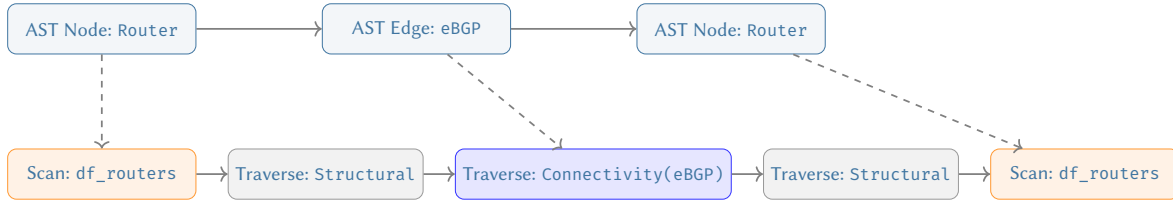
Figure 34. AST Compilation to Execution Plan. The semantic Cypher AST (top) is mathematically expanded by the Query Planner into a deterministic traversal plan (bottom) across the normalized Endpoints graph and partitioned DataFrames.
