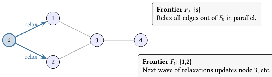
Figure 22. GPU SSSP as wavefront relaxation. Each iteration processes a frontier of active vertices and relaxes outgoing edges in parallel. This maps naturally onto GPU execution when adjacency is stored in compact buffers.
