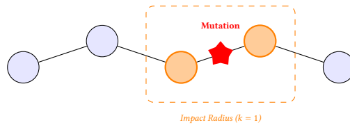
Figure 16. Incremental Validation via Impact Radius. By identifying the nodes physically and logically adjacent to a mutation, NTE avoids the O(V) cost of global policy re-evaluation.
