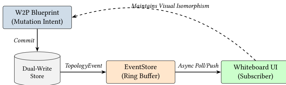
Figure 50. The Reactive Event Pipeline. Structural and relational changes are emitted as typed events, which bridge the physical storage layer back to the visual Blueprint domain.
