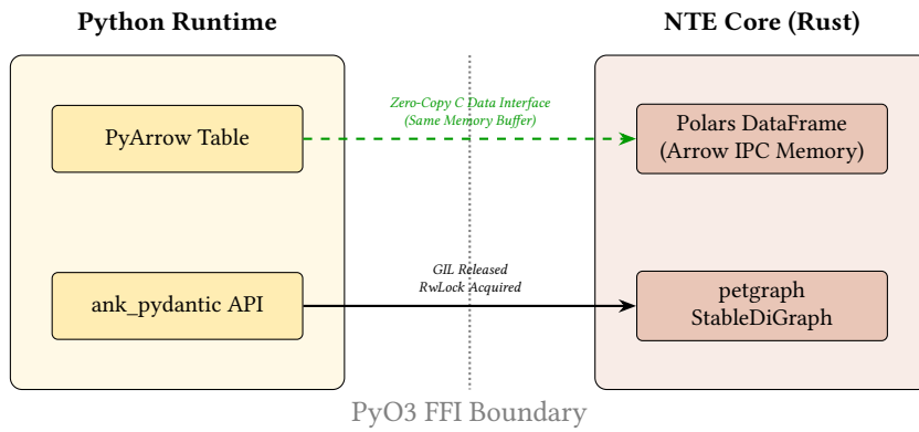
Figure 30. The FFI Zero-Copy Boundary. Unlike traditional RPC-based graph databases, NTE embeds directly in the Python process. The Arrow C Data Interface allows Python tools to read the Rust memory buffers without any serialization overhead.
