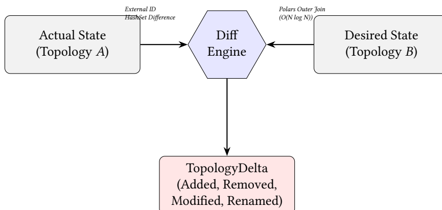
Figure 45. Topology Diffing Pipeline. The engine combines structural set operations with vectorized relational joins to identify deviations between Actual and Desired network states.
