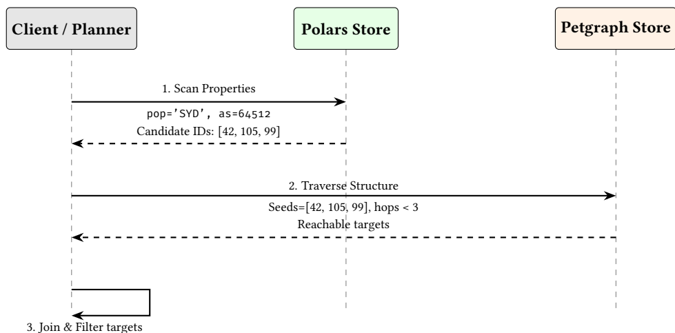
Figure 40. The Filter-First Pipeline. Relational scans prune the search space before expensive graph traversals are initiated.
