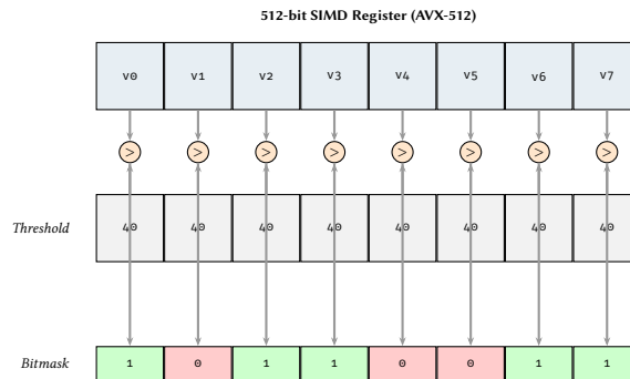
Figure 28. Hardware-Level Predicate Evaluation. A single AVX-512 instruction evaluates multiple property values in parallel, producing a bitmask that drives the subsequent graph traversal filter.
