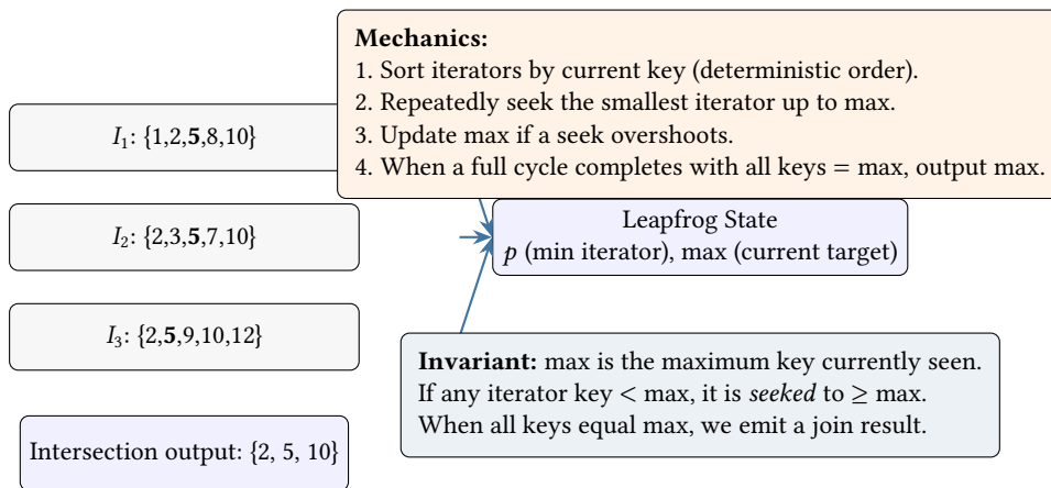
Figure 17. Leapfrog Triejoin as a stateful multi-way intersection. The algorithm maintains a single target (max) and advances the smallest iterator until all iterators align on the same key. This avoids intermediate-result explosion on cyclic patterns by intersecting all constraints simultaneously.
