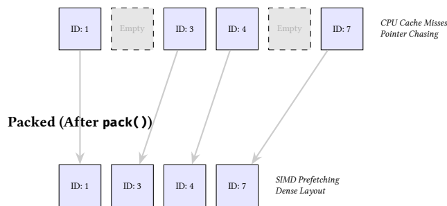
Figure 27. Memory Defragmentation (Graph Packing). The pack() operation removes tombstone slots from the internal adjacency arrays, restoring linear CPU cache locality and reducing memory overhead.
