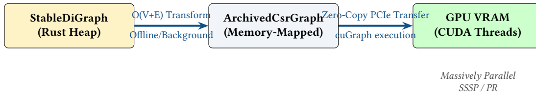
Figure 47. The Graph-to-GPU Pipeline. Because pointer-based graphs cannot be sent to the GPU, the adjacency list is serialized into a flattened Compressed Sparse Row (CSR) structure, which is then DMA-transferred to the GPU for parallel analytics.
