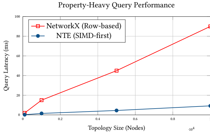
Figure 60. Scaling Performance: NTE vs. NetworkX for complex property filters. NTE’s Polars-backed SIMD scans maintain linear scaling with a significantly lower constant factor compared to row-based alternatives.
