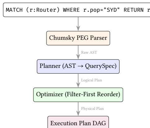
Figure 39. The NTE-QL compilation pipeline. String queries are parsed, converted into programmatic QuerySpec structures, and fed into the same optimizer as the Python APIs.
