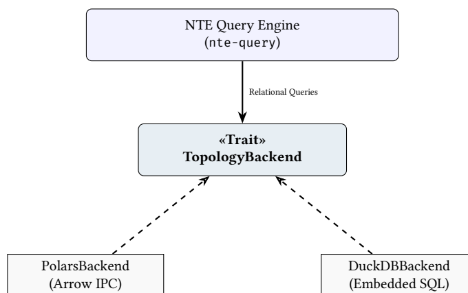
Figure 31. Trait-Based Abstraction. The core query engine interacts only with the TopologyBackend interface, allowing the physical columnar storage (Polars vs. DuckDB) to be swapped at compile time.
