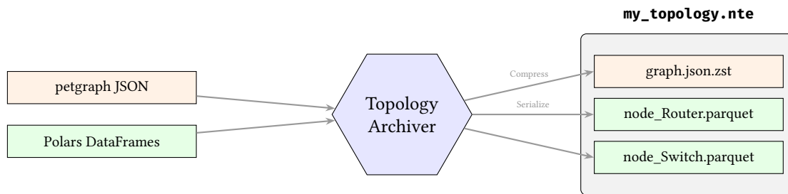
Figure 44. The .nte archive format. Structural graph data is compressed via zstd, while DataFrames are serialised directly to columnar Parquet files, all packaged into a standard ZIP archive.
