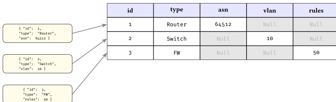
Figure 26. The Wide-Column Sparsity Matrix. Heterogeneous JSON properties are flattened into a single wide DataFrame . Arrow’s validity bitmaps efficiently compress the resulting Null regions.
