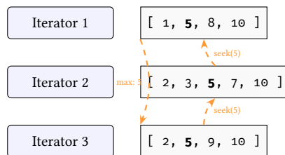
Figure 57. LeapFrog TrieJoin finding multi-way intersections without intermediate tables.
