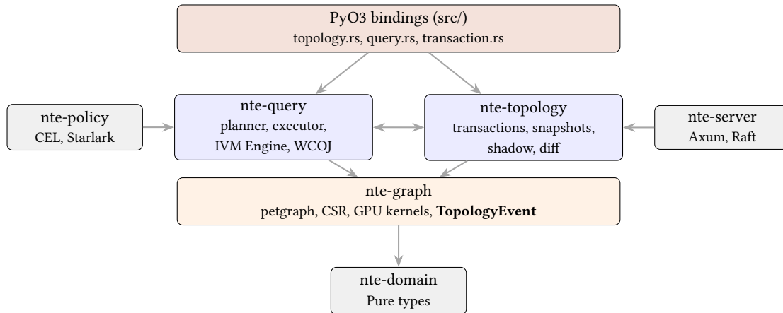
Figure 12. The Layered Crate Architecture. Shared foundation types (Events) are pushed down to nte-graph to enable clean, uni-directional dependency flow between the query engine and topology manager.
