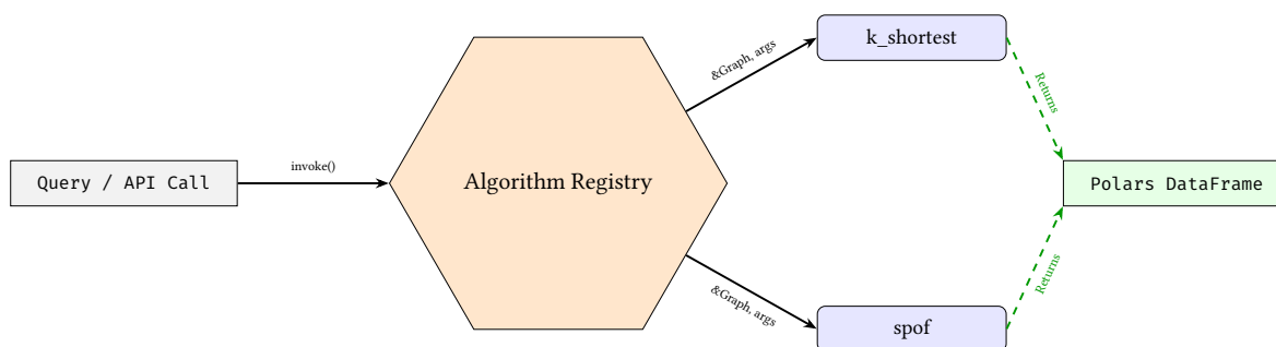
Figure 49. Graph Algorithm Plugin Architecture. Algorithms are invoked by namespace, operate on the shared graph reference, and uniformly return results as Polars DataFrames.
