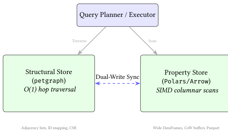
Figure 25. Dual-write architecture synergy. Structural queries target the graph engine, while property-heavy predicates target the columnar store.
