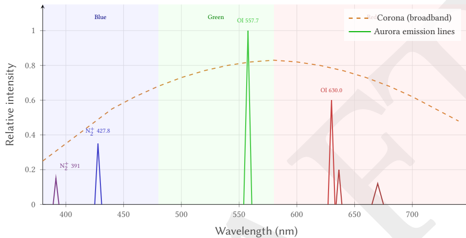
Figure 46. Spectral comparison: aurora produces discrete emission lines (dominant OI green at 557.7 nm, OI red at 630 nm, N 2 + blue at 427.8 nm) while the solar corona emits broadband continuum light. Bayer filter channel boundaries shown as background shading. The green channel’s sensitivity to the dominant 557.7 nm aurora line explains why green clips first.
