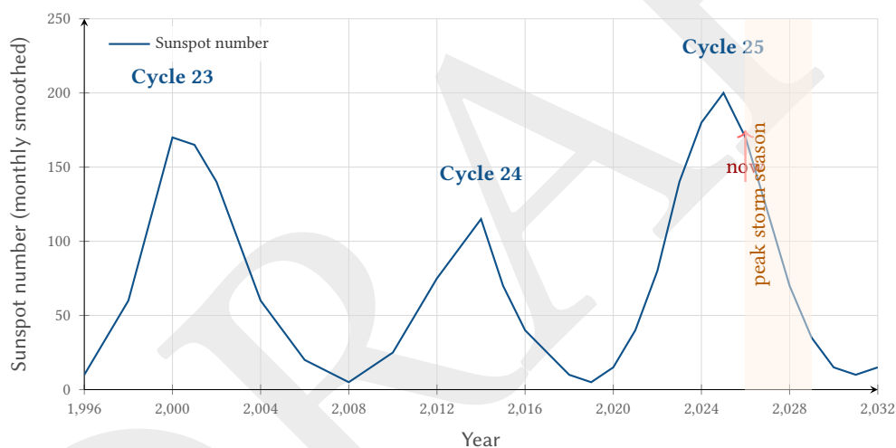
Figure 58. Solar cycle history and projection: Solar Cycle 25 is near its peak in 2025–2026, with the declining phase (2026–2029) historically producing the most intense geomagnetic storms and aurora. This is an optimal window for AuroraPhoto deployment.
