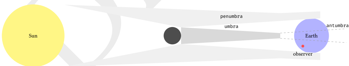
Figure 27. Eclipse shadow geometry (cross-section): the Moon casts an umbral cone (total shadow), penumbral cone (partial shadow), and antumbra (annular shadow region beyond the umbral vertex).
