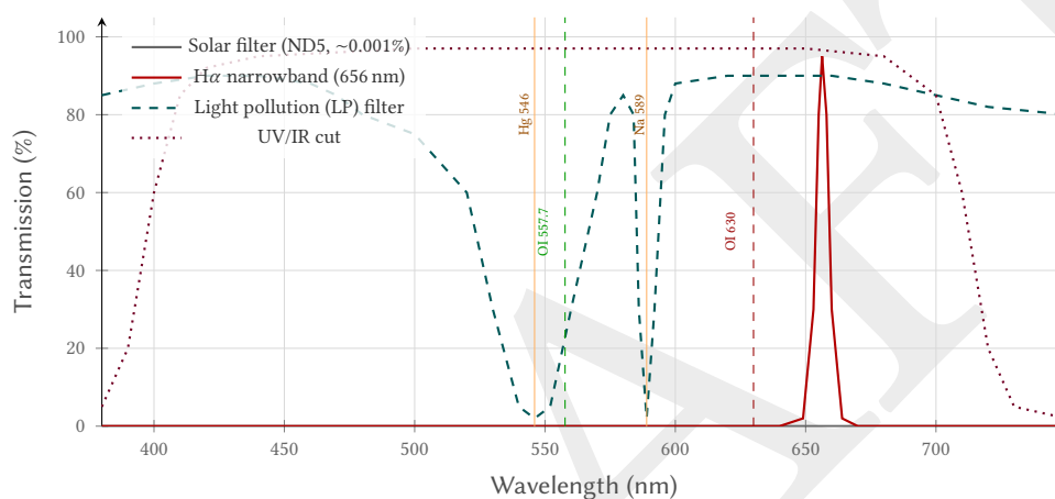
Figure 49. Filter transmission profiles: solar ND5 filters attenuate by ~5 orders of magnitude for safe partial-phase imaging; H \alpha narrowband isolates chromospheric emission; light pollution filters reject sodium and mercury street lighting while passing aurora wavelengths.
