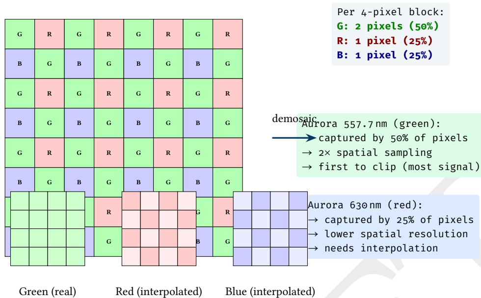
Figure 76. Bayer CFA pattern: green pixels outnumber red and blue 2:1. For aurora imaging, the dominant 557.7 nm green emission lands on 50% of the sensor pixels, giving higher effective resolution but also making green the first channel to clip. Demosaicing interpolates the missing color values, which can introduce artifacts at sharp aurora boundaries.
