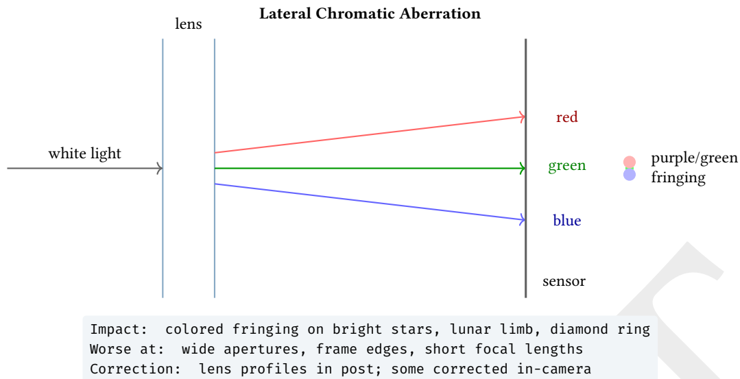
Figure 80. Lateral chromatic aberration: different wavelengths focus at slightly different positions, creating color fringing on high-contrast edges. Particularly problematic for diamond ring shots and the lunar limb during partial phases.
