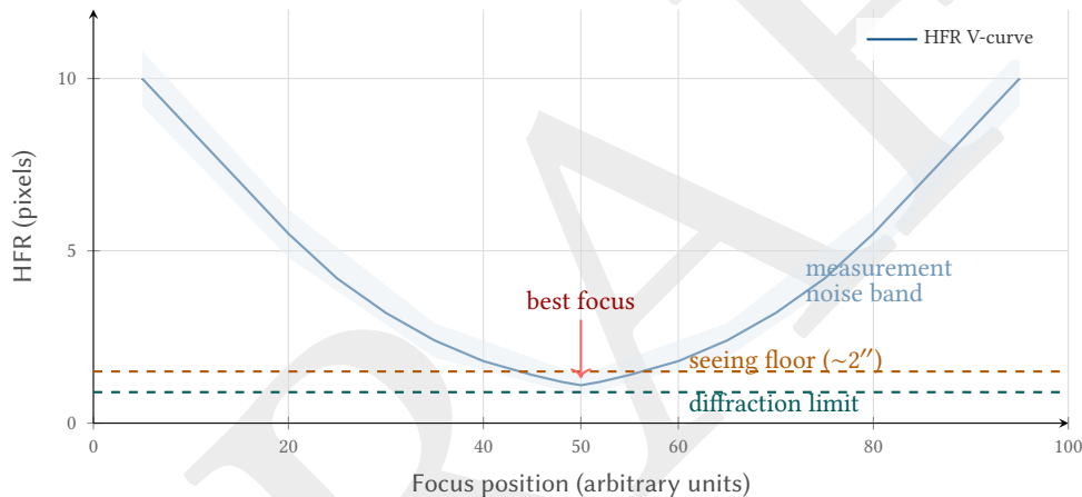
Figure 66. Focus V-curve: HFR follows a characteristic V-shape with minimum at best focus. The shaded band represents measurement noise (from photon statistics and sky background). The diffraction limit and seeing floor impose a hard minimum that even perfect focus cannot surpass.
