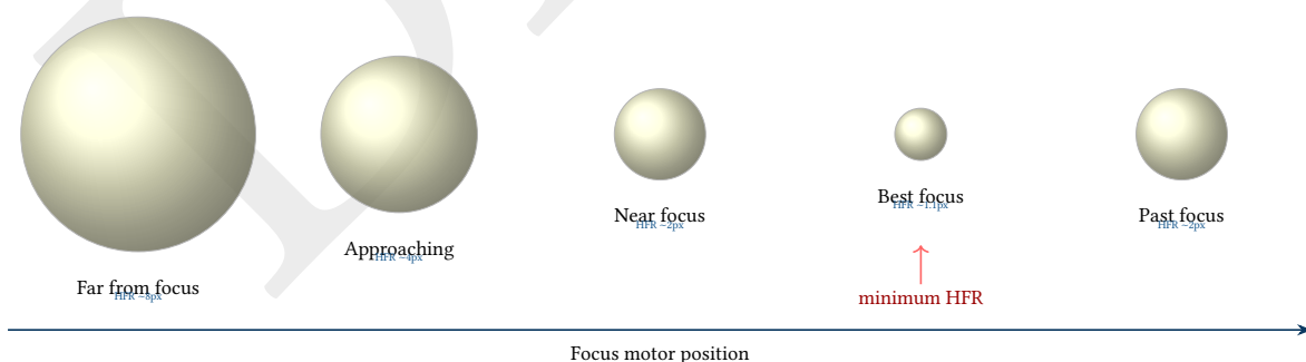
Figure 67. Visual representation of star images at different focus positions: defocused stars appear as large discs; the focus loop minimizes disc size (HFR) by stepping the motor to the V-curve minimum.
