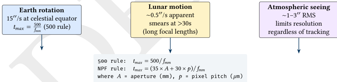
Figure 39. Three sources of motion blur in astrophotography, with formulas for maximum exposure before star trailing becomes visible.
