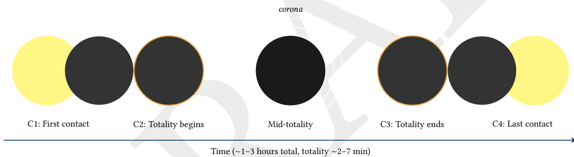
Figure 26. Solar eclipse contact sequence: C1 (first external tangency), C2 (totality onset), mid-totality with corona visible, C3 (totality end), C4 (last external tangency).
