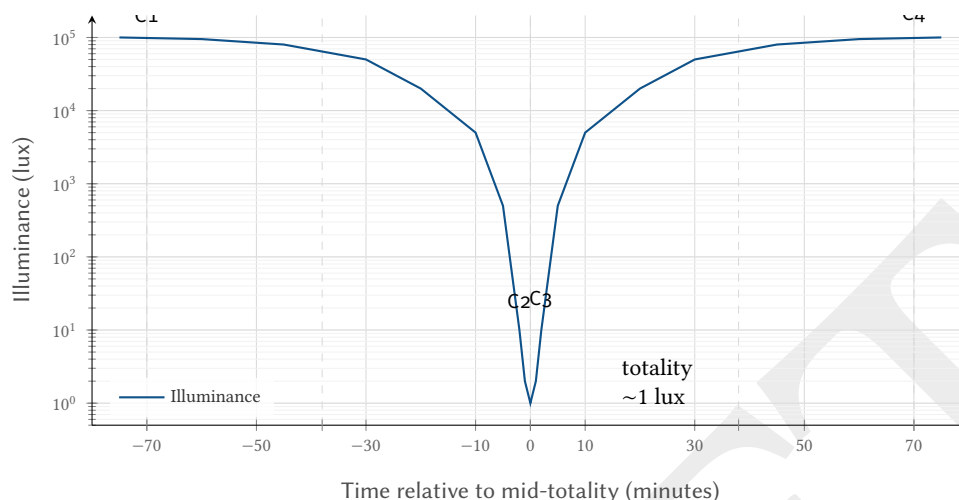
Figure 32. Solar eclipse illuminance curve (log scale). The drop from ~100,000 lux to ~1 lux occurs over just a few minutes around C2/C3, requiring a ~17 EV stop adjustment.
