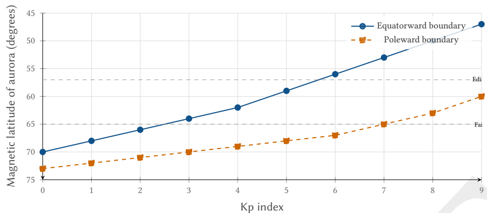
Figure 57. Auroral oval latitude vs. Kp index: higher geomagnetic activity pushes the oval equatorward. A site at 65° magnetic latitude sits under the oval for most Kp values; a site at 57° requires Kp \geq 6 for overhead aurora.
