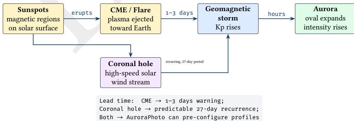
Figure 59. Solar-terrestrial chain: two pathways from solar activity to aurora. CMEs provide 1–3 days warning; coronal hole streams recur on a ~27-day solar rotation period, enabling advance planning.
