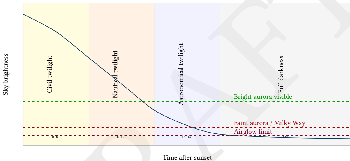
Figure 52. Twilight sky brightness progression: civil twilight (Sun 0–6° below horizon) is too bright for most astrophotography; nautical twilight allows bright aurora detection; full darkness (Sun >18° below) is needed for faint targets. AuroraPhoto should use solar depression angle to select initial exposure profiles.
