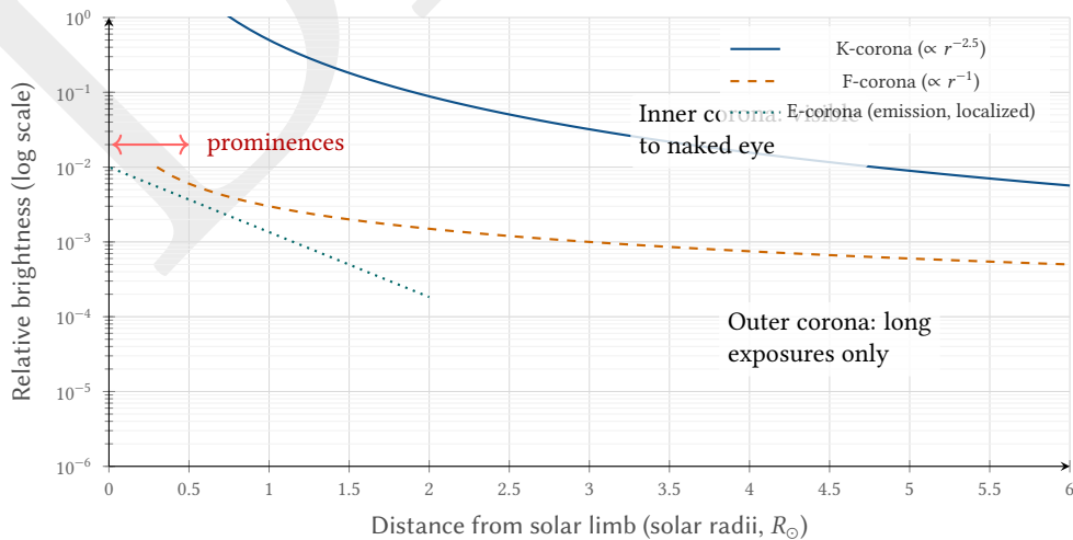
Figure 42. Corona radial brightness profile: the K-corona (electron-scattered) dominates the inner region and drops steeply ( \sim r^{-2.5} ), while the F-corona (dust-scattered) dominates at larger distances with a shallower decline. This radial gradient is the physical reason the dynamic range exceeds 12 EV stops.
