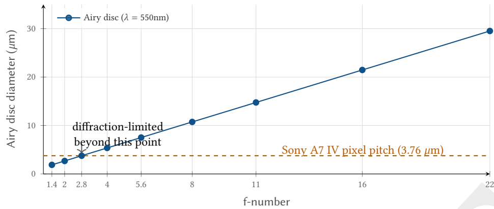
Figure 38. Diffraction-limited resolution vs. f-number: the Airy disc diameter grows linearly with f-number. Beyond the crossover with the sensor pixel pitch, further stopping down reduces resolving power.
