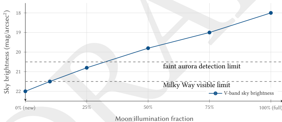
Figure 31. Sky brightness vs. moon illumination fraction. Lower magnitude values (top of plot) indicate brighter skies. Faint aurora and Milky Way structure become invisible as the sky brightens beyond their contrast limits.
