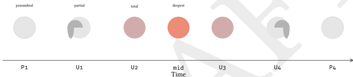
Figure 29. Lunar eclipse stage sequence: the Moon's appearance progresses from subtle penumbral darkening through partial shadow entry to deep red totality and back.
