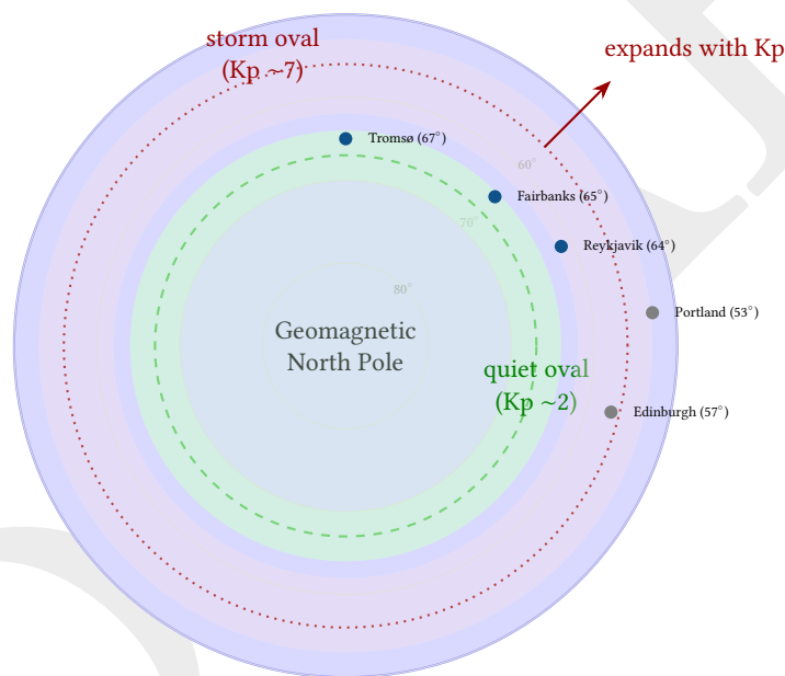
Figure 56. Auroral oval (polar view): during quiet conditions ( K_p \sim 2 ) the oval sits at \sim 65\text{--}70^\circ magnetic latitude; during geomagnetic storms ( K_p \sim 7+ ) it expands equatorward, making aurora visible from mid-latitudes. AuroraPhoto deployments at sites within the quiet oval will see aurora most frequently.
