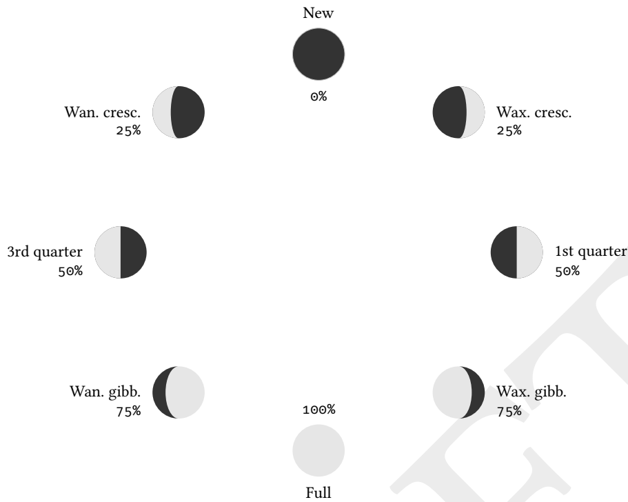
Figure 30. Lunar phase cycle with approximate illumination percentages. Each phase corresponds to a different sky brightness level and thus different imaging constraints.
