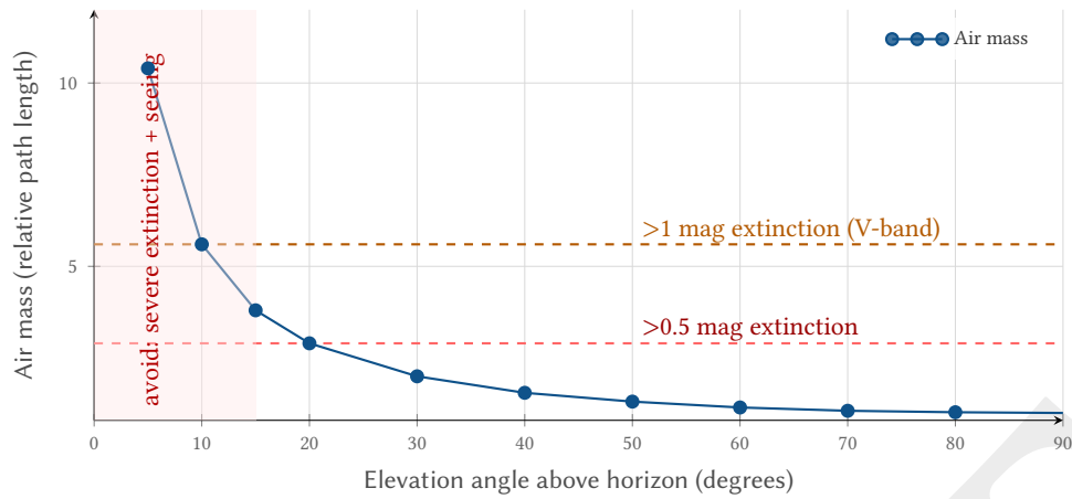
Figure 51. Air mass vs. elevation angle: atmospheric path length increases dramatically below 20° elevation, causing extinction (brightness loss), reddening, and degraded seeing. Targets below ~15° suffer severe quality penalties.
