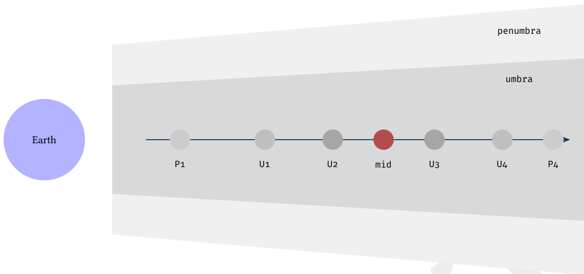
Figure 28. Earth shadow geometry: the Moon traverses the penumbral and umbral cones. P1/P4 mark penumbral entry/exit; U1–U4 mark umbral contacts; mid-eclipse occurs at deepest immersion.
