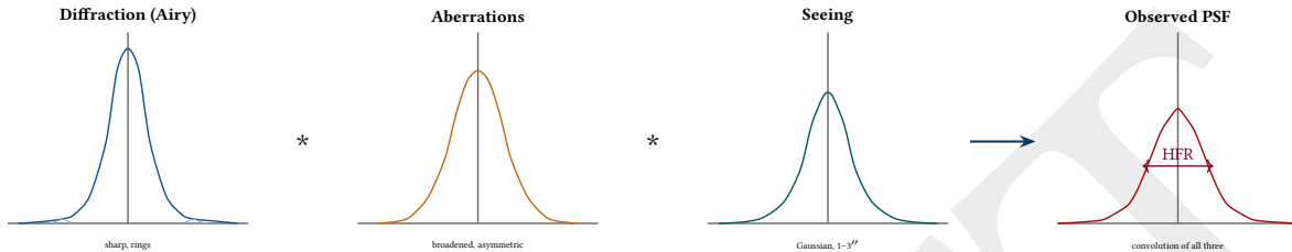
Figure 65. Star PSF composition: the observed profile is the convolution (*) of diffraction (Airy pattern), optical aberrations (lens-dependent), and atmospheric seeing (Gaussian). HFR measures the half-light radius of this combined profile.
