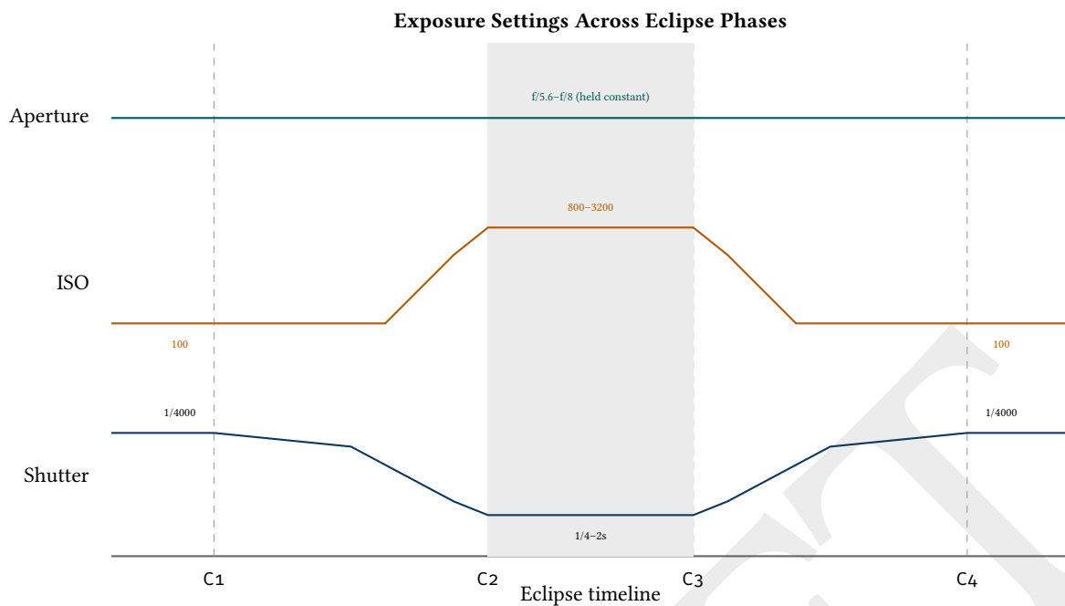
Figure 34. Multi-track exposure timeline: shutter speed and ISO ramp dramatically around C2/C3 while aperture is held constant to maintain optical quality.
