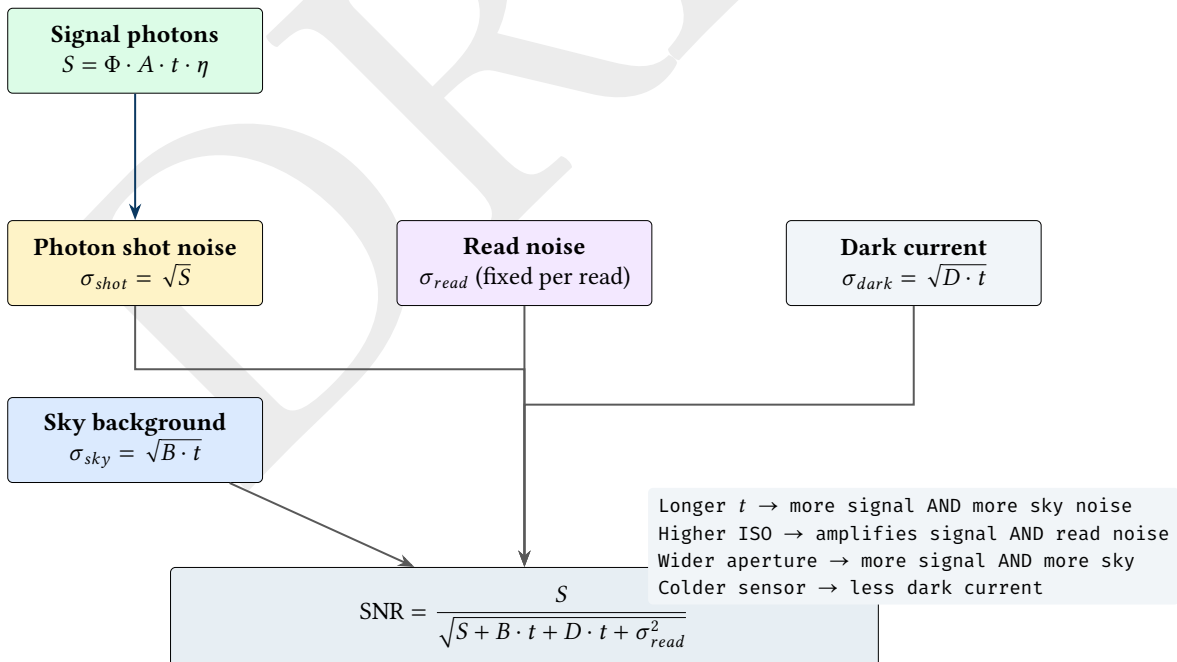
Figure 61. SNR model: signal is proportional to aperture area, exposure time, and quantum efficiency. Total noise combines photon shot noise, read noise, dark current, and sky background in quadrature. This model explains every exposure trade-off in the system.
