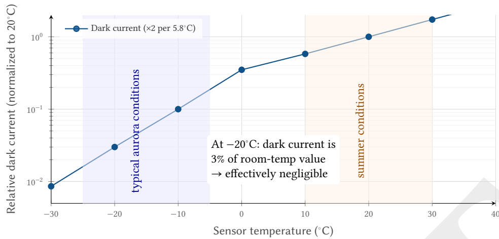
Figure 78. Dark current vs. sensor temperature: the exponential relationship ( \times 2 per \sim 5.8^\circ\text{C} ) means cold-weather aurora shooting at -20^\circ\text{C} has \sim 30\times less dark current than room temperature. This is a significant advantage for long exposures.
