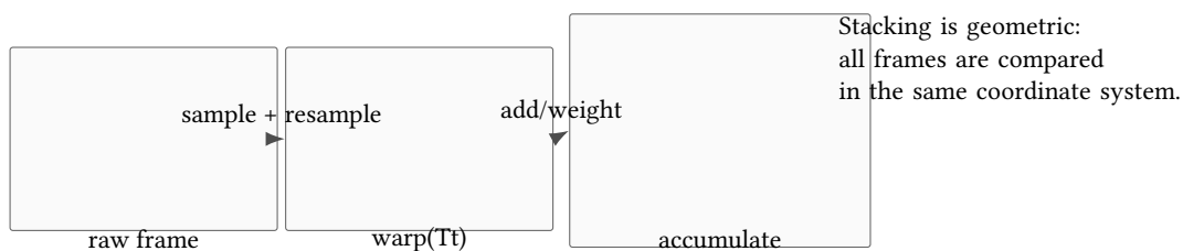
Figure 9. Geometric stacking: warp into the reference coordinate system before accumulation.
