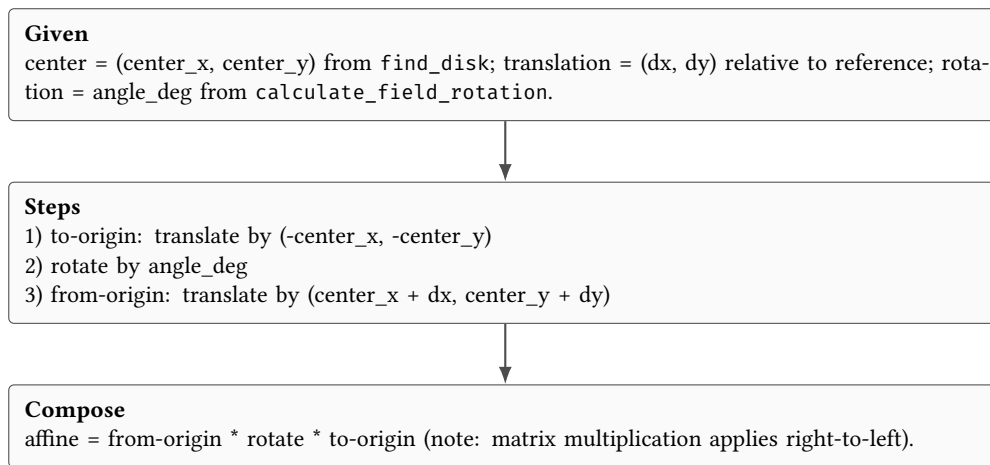
Figure 8. Worked example: how a per-frame affine transform is constructed.
