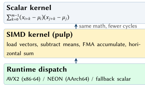
Figure 6. SIMD acceleration strategy. pulp [0] selects an optimal vectorised implementation at runtime while preserving a scalar fallback path.
