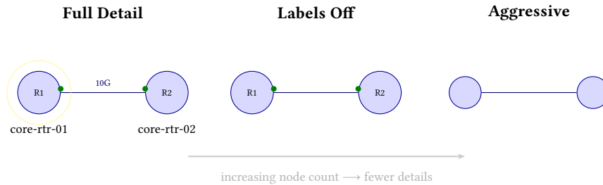
Figure 42. Level of detail (LOD) progressive suppression. As topology size grows past profile thresholds, labels, edge labels, interface markers, and visual effects are progressively hidden to maintain render performance and visual clarity.
