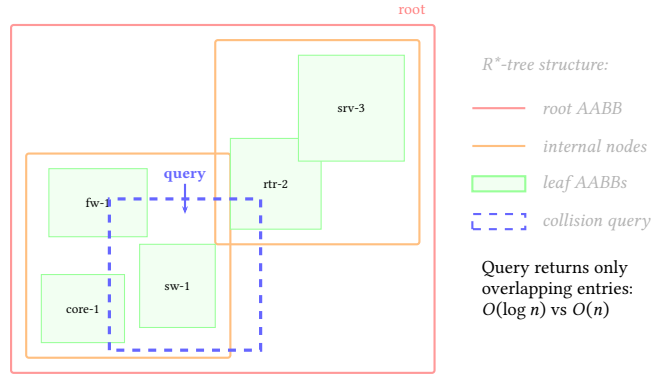
Figure 30. R*-tree spatial index for label collision detection. Occupied regions (node shapes, existing labels, edge exclusion zones) are inserted as axis-aligned bounding boxes. A candidate label position is tested by querying the tree for intersections— O(\log n) per query vs. O(n) brute force.
