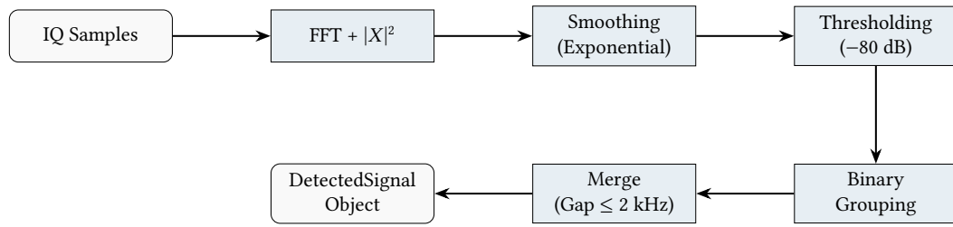
Figure 3. Signal detection pipeline. Raw samples are converted to power spectra, smoothed, and thresholded to produce discrete signal objects.
