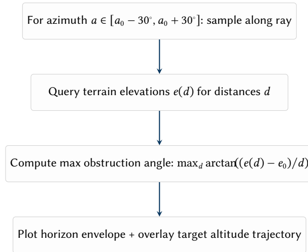
Figure 9. Horizon obstruction estimation pipeline used for the trajectory plot.
