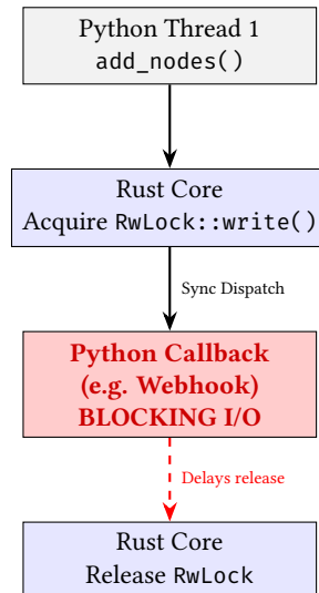
Figure 31. The Event Callback Danger Zone. Synchronous callbacks hold the engine’s global write lock. Future versions will move to a lock-free async queue design.
