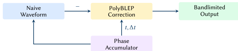
Figure 5. PolyBLEP anti-aliasing: the correction term is subtracted from the naive waveform at phase discontinuities.
