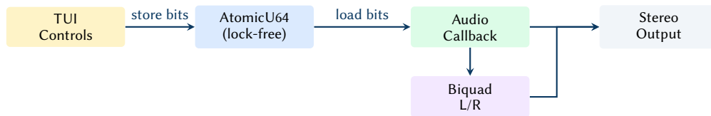
Figure 13. Lock-free live parameter path: the TUI stores f64 bit patterns into atomics; the audio callback loads them each block and updates the biquad filter only when thresholds are exceeded.
