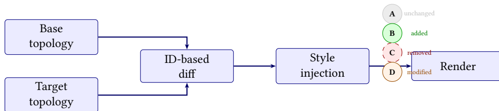
Figure 40. Topology diff pipeline. Nodes and edges are matched by ID between base and target topologies. Changes are classified and color-coded in the rendered output: green (added), red/dashed (removed), amber (modified), gray (unchanged).
