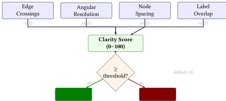
Figure 48. Clarity score composition and CI/CD integration. Four equally-weighted aesthetic factors are combined into a single 0–100 score. CI pipelines can gate on a configurable threshold (default: 85).
