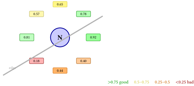
Figure 34. Scoring function applied to 8 candidate label positions around node N. Position scores (0–1) are color-coded from green (good) to red (poor). The right position wins (0.92); the lower-left loses because a diagonal edge passes through it (score 0.18).
