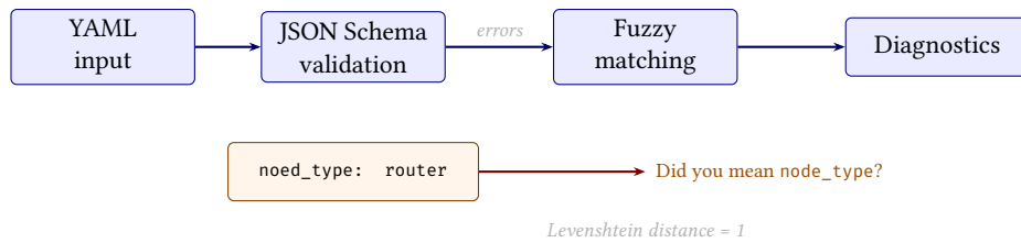
Figure 47. Fuzzy validation pipeline. YAML fields are validated against a JSON Schema generated from Rust types. Unknown fields are matched against valid field names using Levenshtein distance to produce “Did you mean...?” suggestions.
