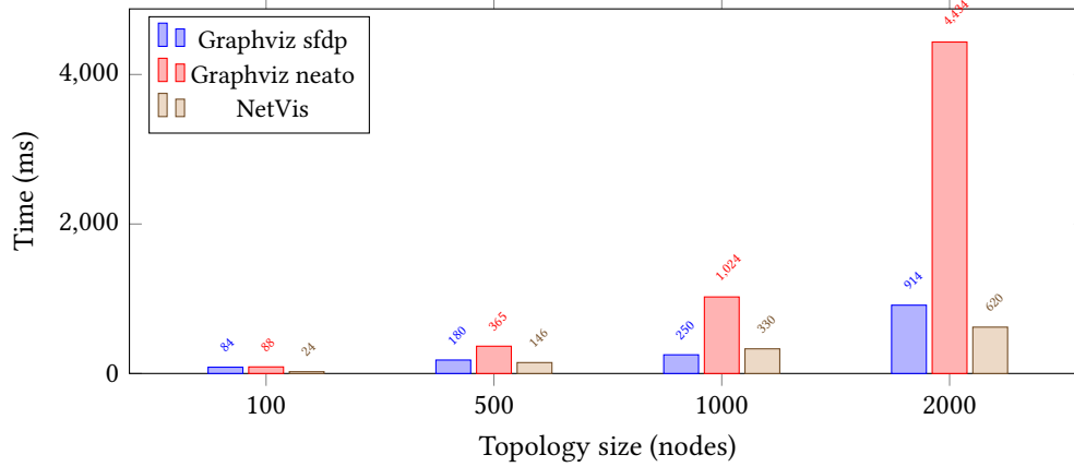
Figure 52. Comparative performance on identical spine-leaf topologies. NetVis includes the full pipeline (layout, labels, styling, SVG render); Graphviz includes layout and SVG output only.
