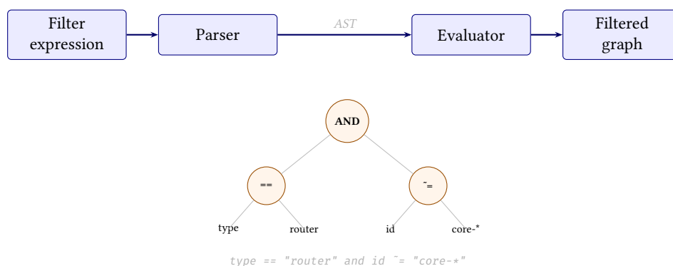
Figure 46. Filter DSL pipeline. A filter expression is parsed into an AST with boolean operators, attribute comparisons, and glob pattern matching. The evaluator walks the AST for each node/edge, retaining only those that satisfy the predicate.
