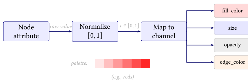
Figure 30. Metric encoding pipeline. A node attribute value is normalized to [0, 1] using min/max bounds, then mapped to one of four visual channels. Color channels use perceptually uniform sequential palettes.
