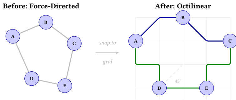
Figure 19. Subway layout: force-directed positions (left) are snapped to an octilinear grid (right). All edges use only 0^\circ , 45^\circ , and 90^\circ segments with at most two bends per edge.
