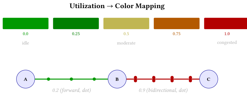
Figure 42. Traffic flow animation. Edge utilization (0.0–1.0) maps to a green–amber–red color ramp. Animated dots travel along the edge path; bidirectional mode shows two opposing dot streams. CSS @keyframes drives the animation in SVG output.
