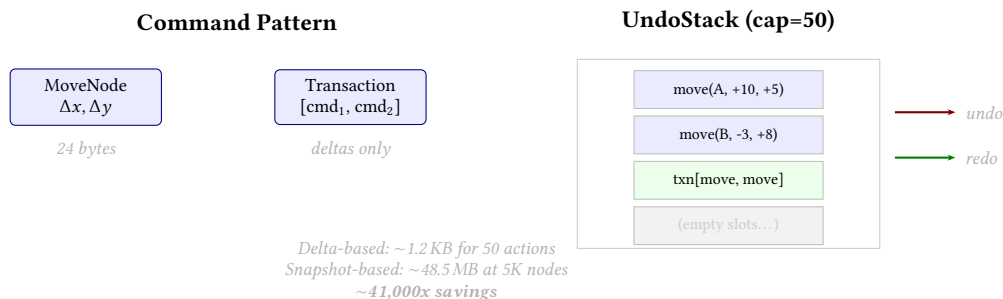
Figure 43. Interactive editor: command pattern with delta-based undo/redo. Each command stores only the change delta (24 bytes for a node move), not a full scene snapshot. The UndoStack with 50-action capacity uses ~41,000x less memory than snapshot-based undo at 5,000 nodes.
