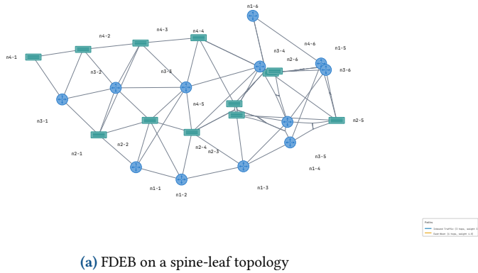
Figure 36. Edge bundling modes. Left: FDEB groups geometrically compatible edges. Right: shared-endpoint mode bundles edges at the hub, fanning out to spokes.
