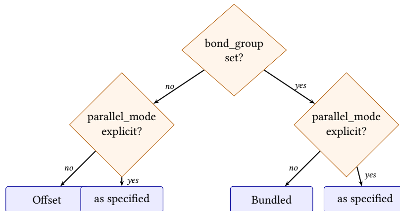
Figure 24. Parallel edge mode selection logic. Bond groups default to Bundled; non-bonded parallel edges default to Offset. An explicit parallel_mode always overrides the default.
