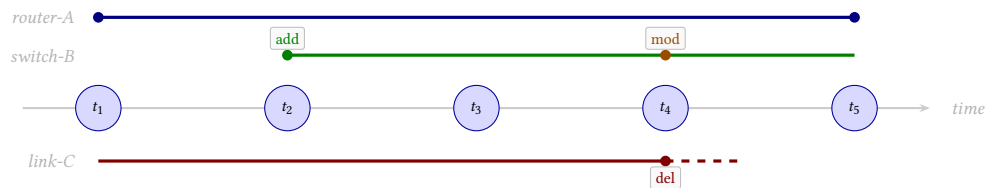
Figure 41. Temporal analysis: entity lifecycle tracking across topology snapshots. Each snapshot ( t_1 – t_5 ) is a YAML file. The timeline module traces first appearance (add), attribute changes (mod), and removal (del) for every node and edge.
