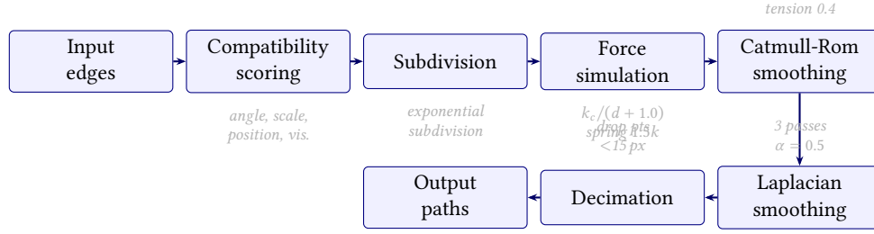
Figure 35. FDEB bundling pipeline. Compatibility scoring determines which edge pairs attract each other; force simulation pulls compatible edges together; post-processing smooths and decimates the result.
