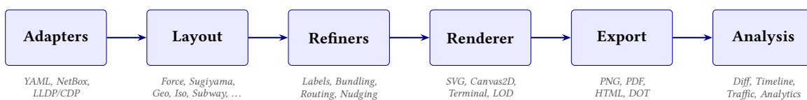
Figure 12. The NetVis six-layer pipeline.
