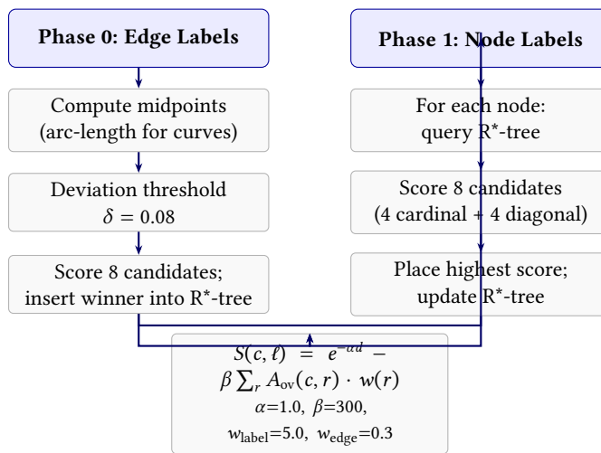
Figure 32. Label placement algorithm. Phase 0 places edge labels first (more constrained by midpoint proximity). Phase 1 places node labels around already-occupied regions. The scoring function penalizes both distance from the owner and overlap with existing geometry.
