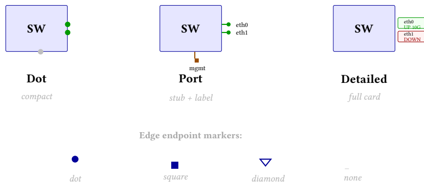
Figure 27. Interface rendering modes. Dot : compact circles on the node boundary. Port : rectangular stubs with labels. Detailed : full interface cards with status and speed. Four marker types control the edge endpoint symbol.
