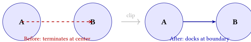
Figure 38. EdgeClippingRefiner: without clipping, edge paths terminate at node centers; with clipping, endpoints dock at the exact node shape boundary, giving correct arrowhead placement regardless of shape.
