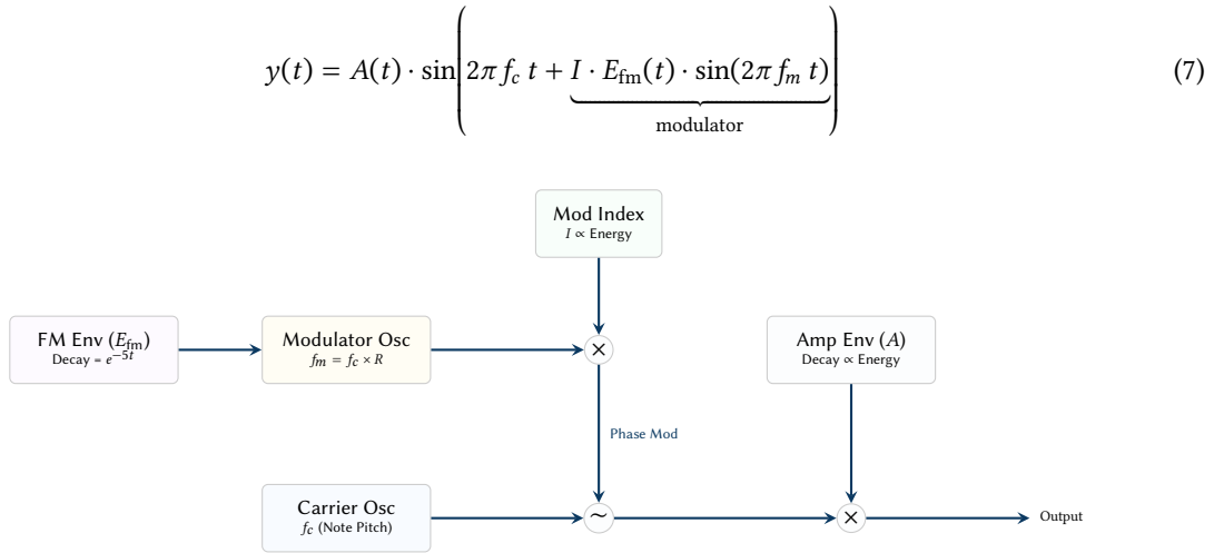
Figure 13. Two-operator FM Synthesis architecture. The modulator oscillator frequency ( f_m ) is a ratio ( R ) of the carrier pitch. The modulation depth (Index I ) is dynamically scaled by the macro energy level, meaning higher energy sections produce much brighter, richer sideband harmonics. The FM envelope ( E_{fm} ) creates a "pluck" or "wow" transient.
