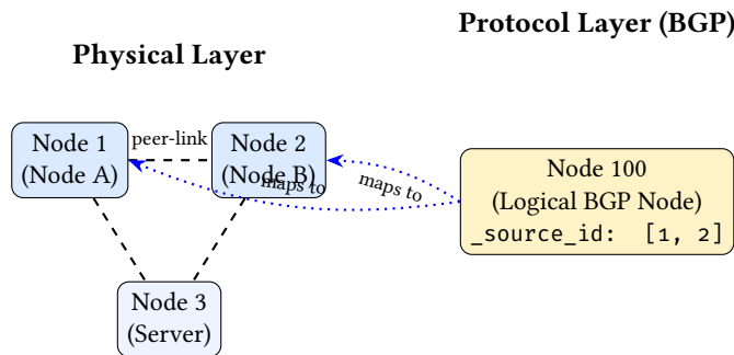
Figure 27. MLAG/vPC topology mapping. Two physical nodes collapse into a single logical protocol node via array _source_id .
