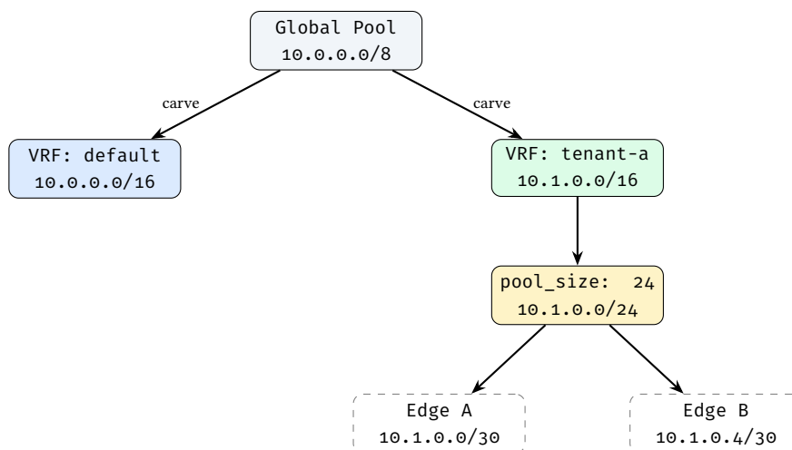
Figure 26. Hierarchical IP pool carving with VRF isolation.
