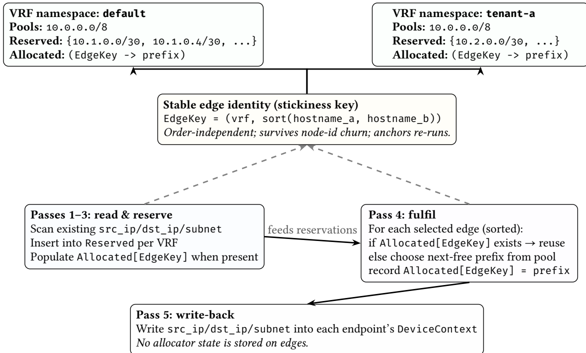
Figure 25. Allocator state model. Allocations are partitioned by VRF and keyed by a stable semantic edge identity (hostnames, not integer IDs). Existing allocations are pre-reserved for stickiness; new prefixes are chosen from the free space within the VRF namespace, then written back to node DeviceContext .
