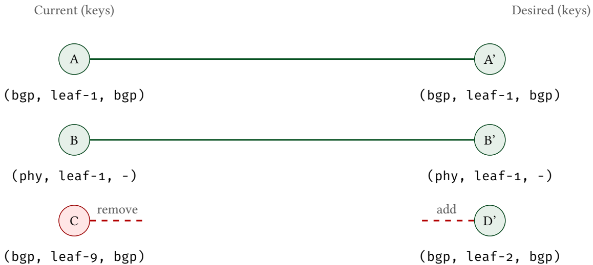
Figure 30. Why semantic keys matter. Matching by integer ID turns benign insertions into widespread “updates”; matching by a composite semantic key isolates changes to the nodes that actually changed.
