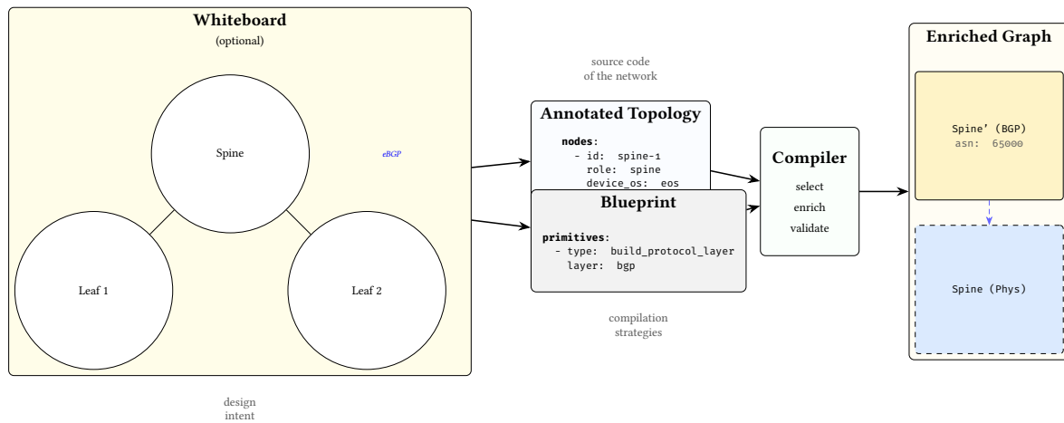
Figure 10. From whiteboard to compiled model. An architect’s visual intent (left, optional) informs both the annotated topology (the network’s “source code”: nodes, roles, sites, properties) and the blueprint (which compilation strategies to apply). Together, these feed the compiler, which produces an enriched, layered graph (right).
