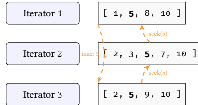
Figure 39. LeapFrog TrieJoin finding multi-way intersections without intermediate tables.
