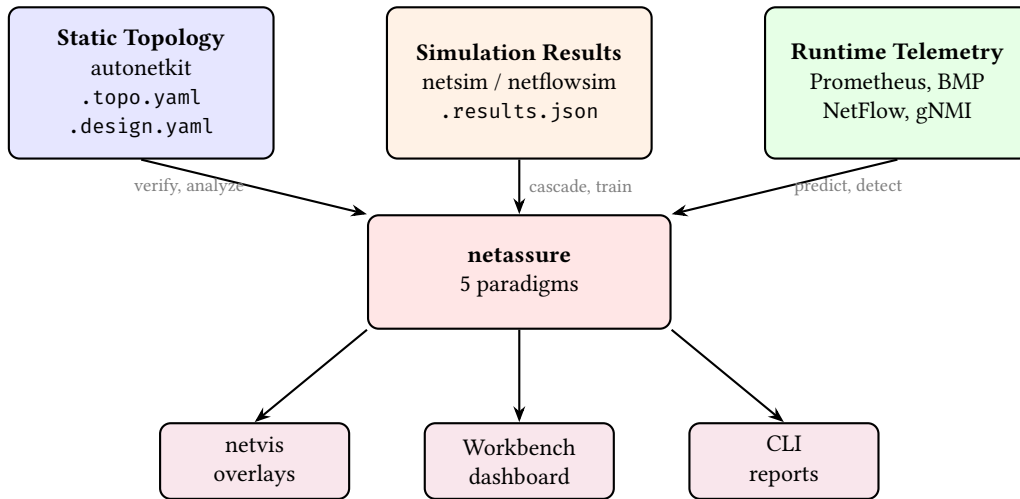
Figure 7. Multi-source analysis data flow: three data sources feed netassure, which produces insights for three consumer types.
