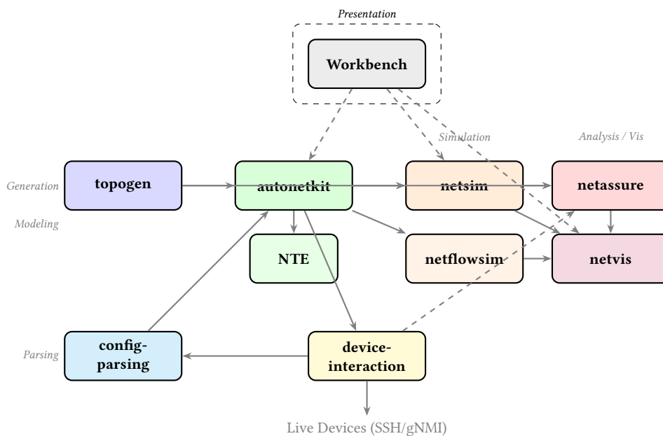
Figure 8. Ecosystem overview: ten tools in architectural layers with data flow arrows. Solid arrows are implemented; dashed arrows are planned.
