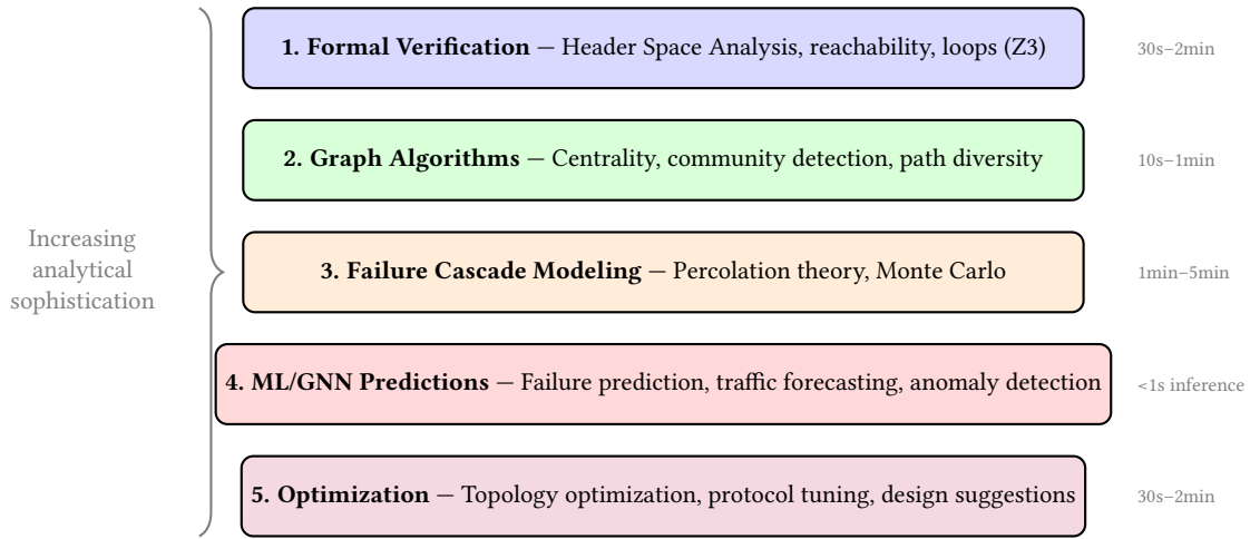
Figure 6. The five analysis paradigms of netassure, with typical compute times.
