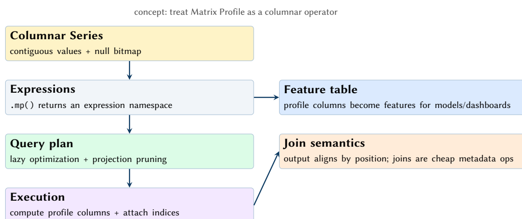
Figure 18. Polars conceptual model. Matrix Profile computation is exposed as a columnar operator: expressions form a plan, Polars optimizes the plan, and execution yields profile/indices as new columns that can be joined into feature tables.
