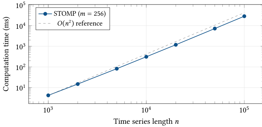
Figure 26. STOMP batch scaling. Measured times track ideal O(n^2) scaling closely across two orders of magnitude.
