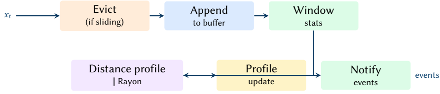
Figure 14. Data flow through append_point . Eviction (orange) only executes in sliding mode. The distance profile computation is parallelised across windows via Rayon.
