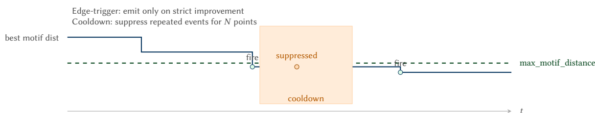
Figure 17. Notification semantics (motifs shown). Events are edge-triggered: a motif event fires only when the global best-so-far distance strictly improves past the configured threshold. A cooldown window suppresses repeated events during rapid convergence.
