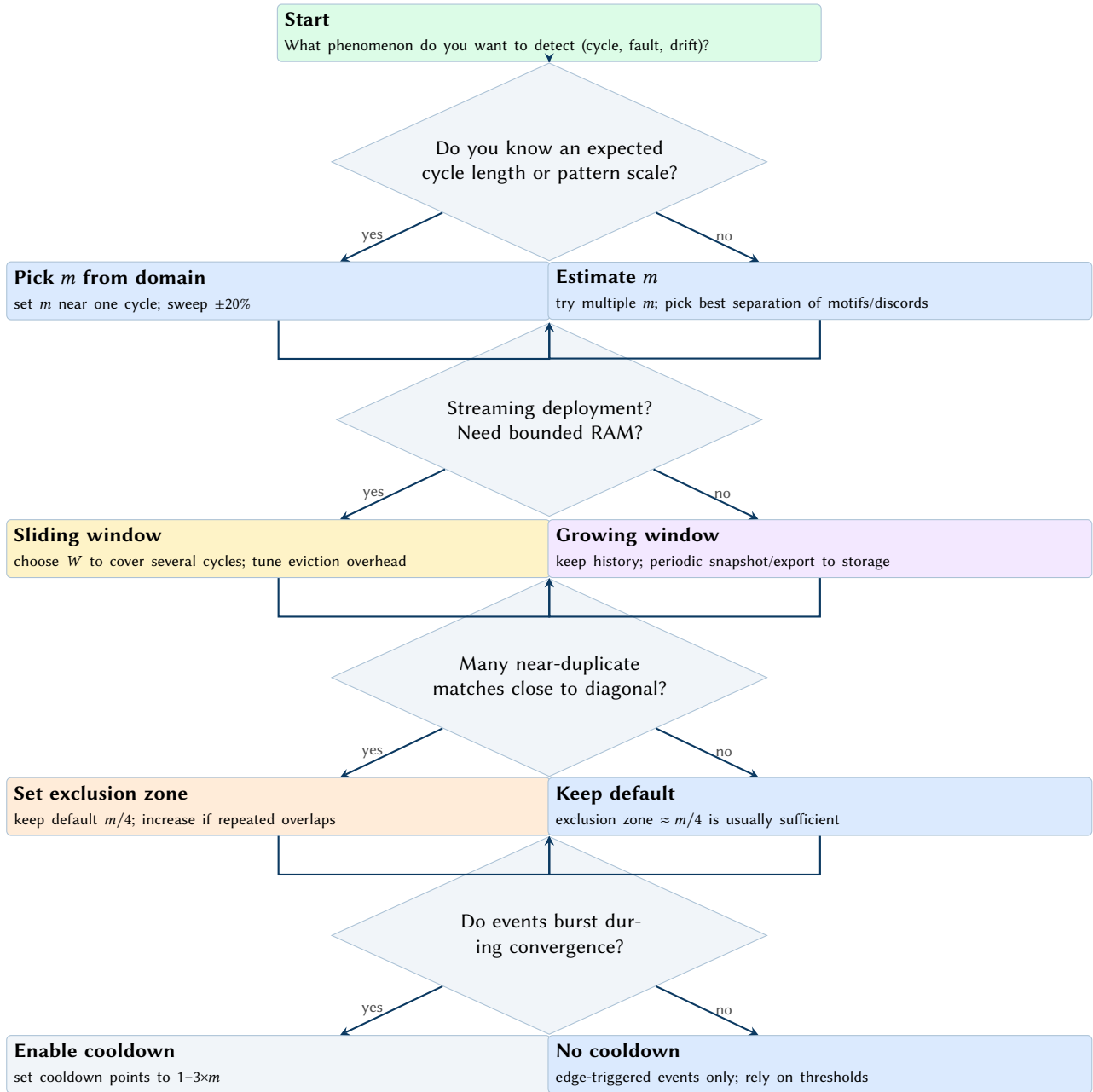
Figure 28. Parameter selection flowchart. Start from domain time scales for m , pick a memory mode (sliding vs growing), keep a conservative exclusion zone, and add cooldown when event streams become noisy.
