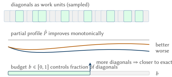
Figure 16. SCRIMP++ anytime intuition. Sampling more diagonals can only improve nearest-neighbour distances, so the approximation refines monotonically as budget increases [6].
