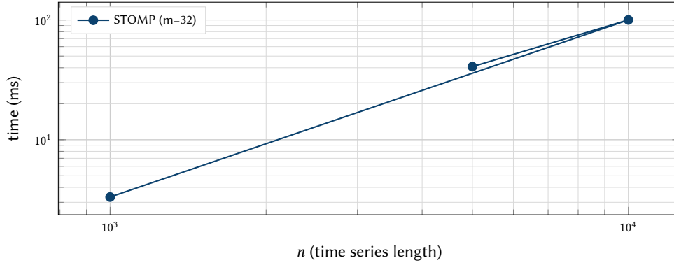
Figure 20. End-to-end STOMP scaling (Criterion, representative). Log-log axes emphasise the rapid growth in compute cost with n for exact batch joins. Values match Table 3.
