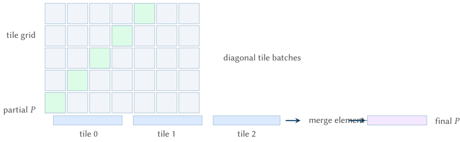
Figure 11. Tiled STOMP for out-of-core datasets. stomp_tiled processes the distance matrix in memory-bounded tiles, producing partial profiles that are merged via an element-wise minimum reduction to yield the final Matrix Profile.
