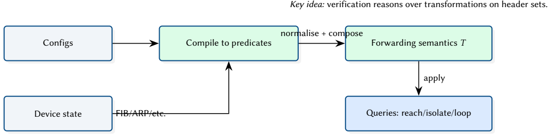
Figure 7. Conceptual compilation pipeline from configuration artefacts to forwarding semantics.
