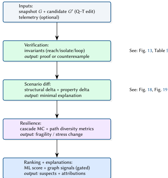
Figure 2. End-to-end case study thread: one topology edit produces verification, impact, resilience, and ML artefacts.
