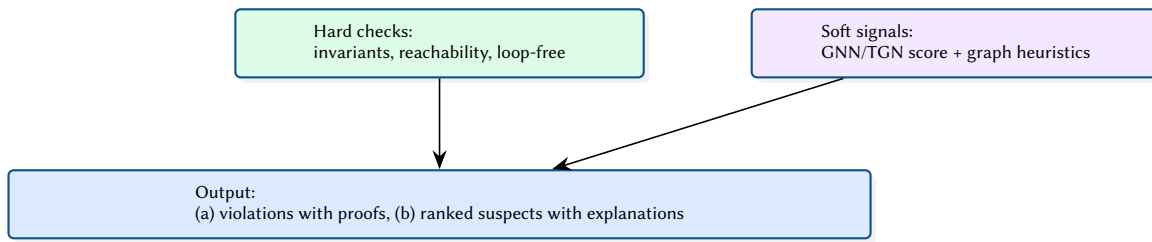
Figure 30. Fusion concept: correctness gates (hard) plus prioritisation signals (soft).
