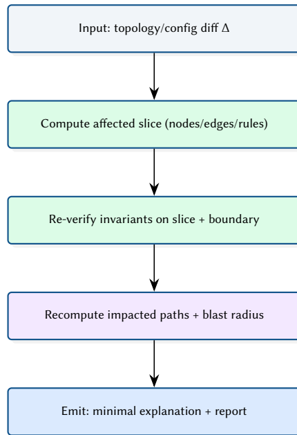
Figure 23. Conceptual incremental update path: restrict recomputation to an affected slice when analysing diffs.
