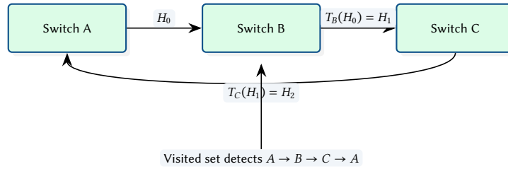
Figure 8. Conceptual header-space propagation and loop detection.
