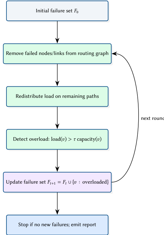
Figure 14. Round-based cascade progression used in the Monte Carlo simulator.
