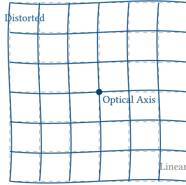
Figure 25. Visualization of SIP polynomial distortion warping the linear TAN projection grid away from the optical axis.
