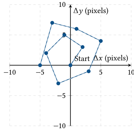
Figure 22. A pseudo-random Dither map over 10 exposures. Between each frame, the mount is commanded to shift slightly. While the stars are re-aligned during registration, the fixed-pattern sensor noise is decoupled and scattered across the grid, allowing the sigma-clipper to successfully reject it.
