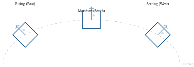
Figure 37. The field rotation effect on an Alt-Az mount. The target (represented by the sensor frame) rotates relative to the celestial field as it traverses the sky, requiring active mechanical derotation for long exposures.
