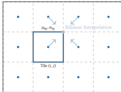
Figure 15. Background estimation using a local grid. Each tile computes a sigma-clipped mean, which is then bilinearly interpolated across the image to model spatial gradients.
