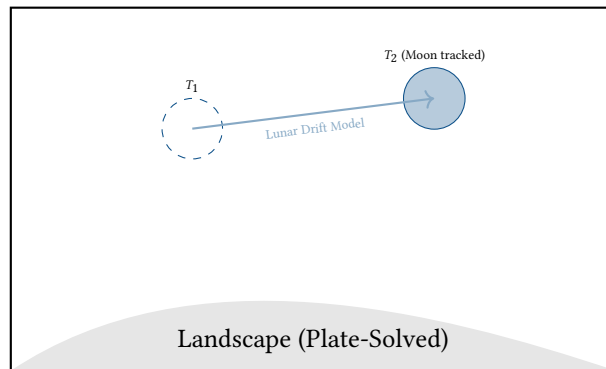
Figure 50. The Eclipse Composite Engine. By plate-solving the wide-field landscape shot to establish a baseline WCS, the system can mathematically superimpose high-resolution, tracked shots of the Moon at their exact predicted celestial coordinates for a given timestamp.
