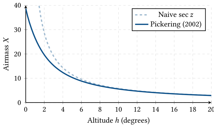
Figure 5. Comparison of airmass models near the horizon. The naive secant approximation diverges to infinity at h = 0^\circ , whereas Pickering's interpolation correctly models atmospheric curvature to match empirical scattering data ( X \approx 38 at the horizon).
