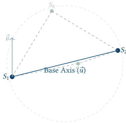
Figure 45. A 4-star geometric “quad” used for blind plate solving. The two most distant stars ( S_1, S_2 ) define a normalized 2D coordinate system ( \vec{u}, \vec{v} ). The internal positions of S_3 and S_4 within this system create a translation-, rotation-, and scale-invariant 4D hash code used to rapidly search the celestial index.
