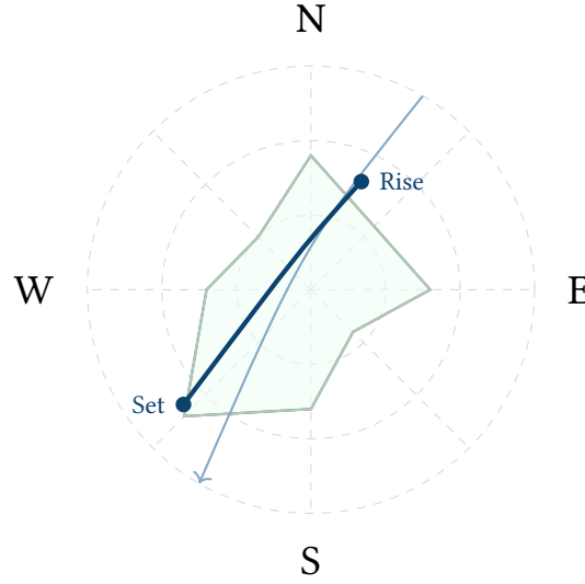
Figure 8. Altitude-Azimuth polar projection (zenith at center, horizon at edge). The shaded polygon represents the local topographical horizon mask (e.g., trees, buildings). The target's nightly arc intersects the mask to compute precise visibility windows.
