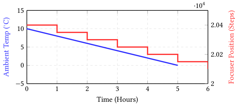
Figure 31. Temperature compensation loop. As the ambient temperature drops steadily (blue), the astro-node daemon autonomously injects computed inward micro-steps to the focuser (red) to maintain critical focus without requiring a sequence-interrupting V-Curve scan.
