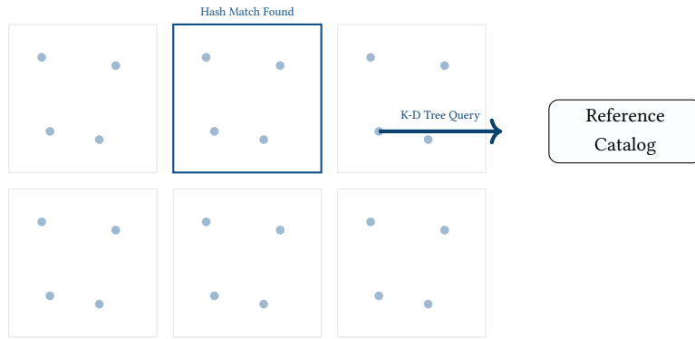
Figure 48. The native plate solver uses quad-hashing (fig. 45) to perform sub-millisecond lookups against a pre-compiled K-D tree of the sky, enabling blind astrometry on devices without internet access or heavy dependencies.
