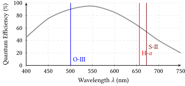
Figure 13. Quantum Efficiency curve of a typical Back-Illuminated (BSI) CMOS sensor. The noise model calculates the expected signal-to-noise ratio by integrating the target’s emission spectrum against the sensor’s specific QE at key narrowband wavelengths (500.7 nm, 656.3 nm, 672.4 nm).
