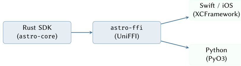
Figure 47. The Mobile Bridge architecture. UniFFI generates the boilerplate required to expose Rust’s rich type system (enums, structs, errors) as idiomatic native objects in Swift and Python.
