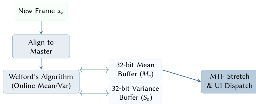
Figure 33. Live Stacking memory architecture. Welford’s single-pass algorithm maintains numerical stability for the running 32-bit mean and variance buffers while preventing Out-of-Memory (OOM) errors during continuous hours-long EAA sessions.
