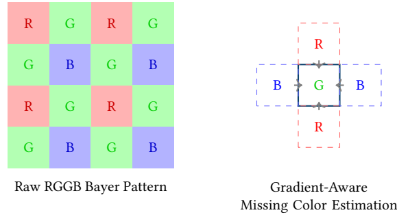
Figure 14. Demosaicing process. The missing color channels at any given pixel are computed using gradient-corrected linear interpolation from neighboring pixels to preserve sharp edges and minimize false-color artifacts.
