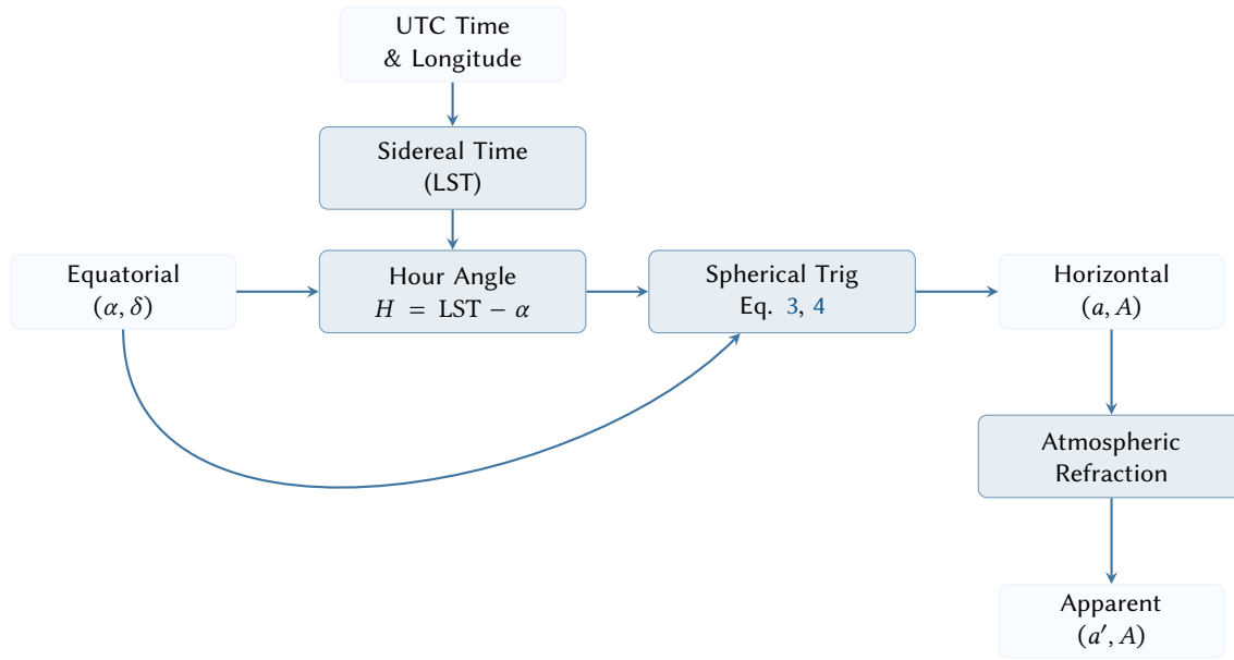
Figure 3. Coordinate transform pipeline mapping equatorial targets to their apparent topocentric positions.
