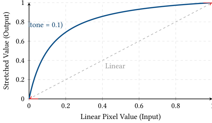
Figure 23. The Midtone Transfer Function (MTF) aggressively expands the dynamic range of the dark background (pulling faint signal up) while compressing the highlights (preventing star cores from blowing out).
