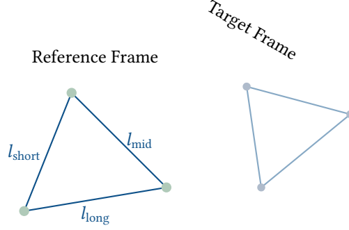
Figure 20. Triangle-similarity matching. The sorted ratios of the sides ( l_{\text{short}}/l_{\text{long}} , l_{\text{mid}}/l_{\text{long}} ) form a scale-, translation-, and rotation-invariant descriptor.
