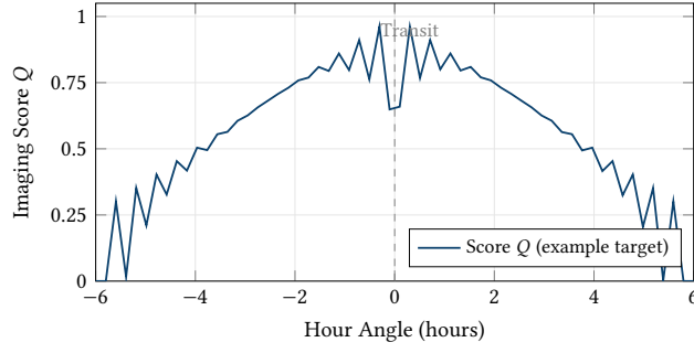
Figure 10. Imaging window score over a night for a representative target at declination +45^\circ . The score peaks near transit (hour angle H = 0 ) where the target reaches maximum altitude and minimum airmass, then decays symmetrically as the target descends toward the horizon.
