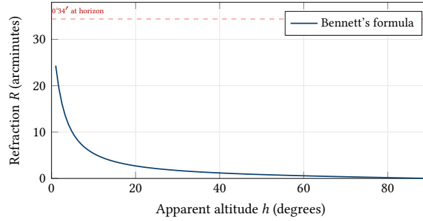
Figure 4. Atmospheric refraction magnitude as a function of apparent altitude using Bennett's formula. Refraction reaches \sim 34' at the geometric horizon, causing objects to appear 0.57^\circ higher than their true position. Above 20^\circ the correction falls below 3' and is often negligible for wide-field framing, but remains significant for rise/set time predictions.
