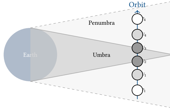
Figure 6. Lunar eclipse shadow geometry showing the Earth’s umbral and penumbral cones. The SDK predicts contact points ( P_1 , U_1 , U_2 , etc.) by stepping through the Moon’s geocentric ecliptic coordinates.
