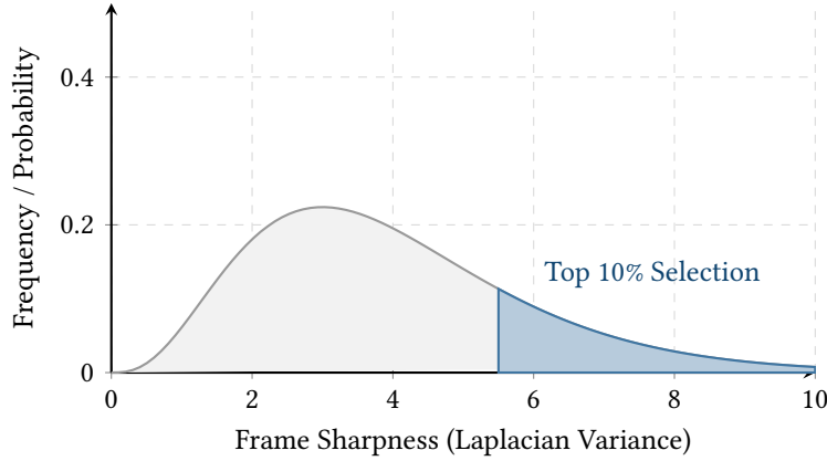
Figure 39. Frame sharpness distribution in a Lucky Imaging sequence. The highly skewed right tail represents the rare frames captured during moments of negligible atmospheric turbulence, which are retained for stacking.
