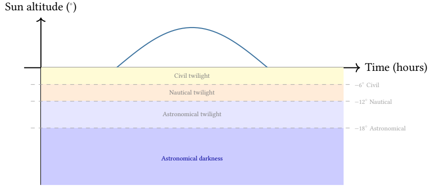
Figure 9. Twilight boundary model. The twilight_times function locates the six solar altitude crossings that delimit civil, nautical, and astronomical twilight, bounding the usable deep-sky imaging window.
