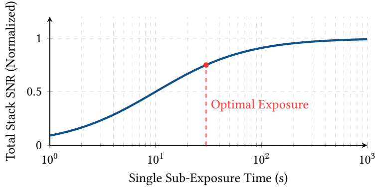
Figure 18. Diminishing returns of sub-exposure time. Once the t_{\text{opt}} threshold is reached (where sky noise swamps read noise), extending the exposure time only increases the risk of ruined frames (e.g., from satellite trails or wind gusts) without improving the final stack's SNR.
