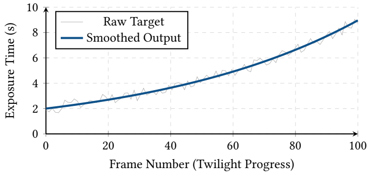
Figure 19. Holy Grail timelapse exposure ramping. The exponential smoothing filter rejects high-frequency noise from passing clouds or atmospheric variations, generating a monotonically increasing exposure schedule that prevents visible flicker.
