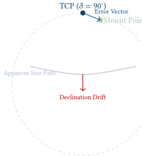
Figure 7. Polar alignment error. A misalignment between the True Celestial Pole (TCP) and the mount’s mechanical polar axis causes stars to exhibit a continuous declination drift over time, which forms the basis of the King drift method.
