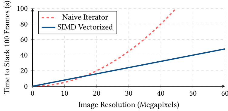
Figure 28. Theoretical scaling performance of Sigma-Clipped stacking. By relying on contiguous memory layouts and SIMD intrinsic vectorization, the stacking module maintains a linear O(N) time complexity, preventing the combinatorial explosion associated with naive per-pixel loop evaluation on large sensors.
