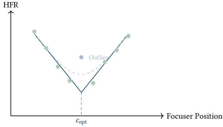
Figure 30. Autofocus V-Curve plotting HFR against focuser position. The robust IRLS fit suppresses the outlier data point.
