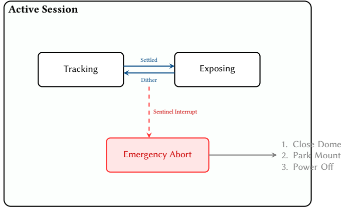
Figure 44. Simplified Harel Statechart of the observatory orchestrator. If the Edge AI Sentinel issues an interrupt (e.g., cloud detected) while the system is nested inside the Exposing or Tracking states, the hierarchy immediately preempts all active futures and transitions to the guaranteed Emergency Abort recovery sequence.
