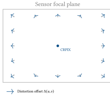
Figure 26. SIP distortion field for a representative wide-field lens exhibiting barrel distortion. Each arrow shows the (\Delta u, \Delta v) pixel correction applied by the A/B polynomials before the linear CD matrix maps to sky coordinates. The correction magnitude is greatest at the corners and falls to zero at the optical centre (CRPIX).
