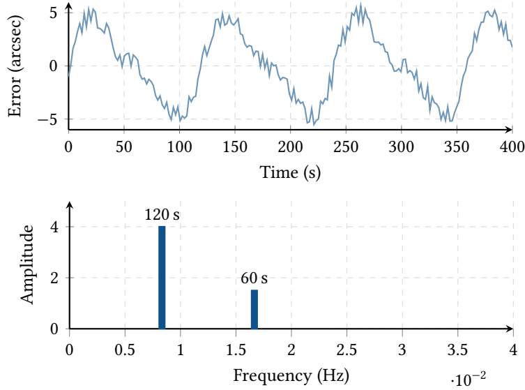
Figure 34. Top: Time-domain simulated tracking error exhibiting a fundamental 120-second worm period and noise. Bottom: FFT frequency-domain spectrum isolating the fundamental frequency (0.0083 Hz) and its first harmonic (0.0166 Hz).
