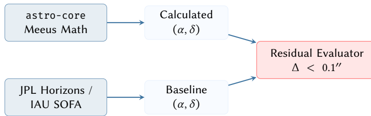
Figure 29. Golden Master CI/CD testing pipeline. The SDK’s coordinate output is dynamically asserted against the gold-standard JPL Horizons ephemeris data [23] to guarantee that the implementation is free from systemic truncations or coordinate frame misinterpretations.
