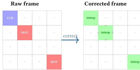
Figure 21. Hot and cold pixel correction in the calibrate module. Defective pixels (red: hot, blue: cold) are identified via MAD-thresholding on the dark master. Each flagged pixel is replaced by the mean of its valid 3 \times 3 neighbours (green), removing permanent sensor defects before registration and stacking.
