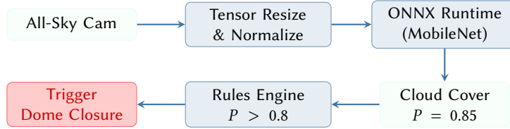
Figure 43. The Sentinel Safety Engine pipeline. Real-time imagery is processed via a cross-platform ONNX inference runtime. The resulting classification probabilities are evaluated against user-defined TOML rules to trigger emergency hardware shutdowns.
