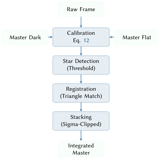
Figure 12. Image processing pipeline from raw sub-exposures to an integrated master frame.
