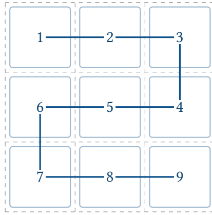
Figure 40. A 3 \times 3 mosaic grid demonstrating the boustrophedon (serpentine) path ordering to minimize mount slew distance.
