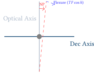
Figure 35. Mount Kinematics. The pointing model corrects for six fundamental mechanical errors: Index errors ( IH, ID ), Polar Elevation/Azimuth ( ME, MA ), Non-perpendicularity ( NP ), and Tube Flexure ( TF ).
