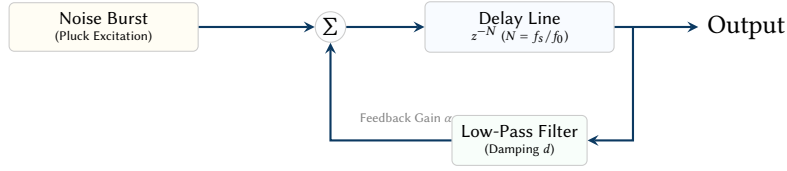
Figure 16. Karplus-Strong physical modeling architecture. A short burst of noise (the "pluck") is fed into a delay line representing the string length. The output is fed back through a low-pass filter, causing higher frequencies to decay faster than fundamental frequencies, realistically simulating a plucked acoustic string.
