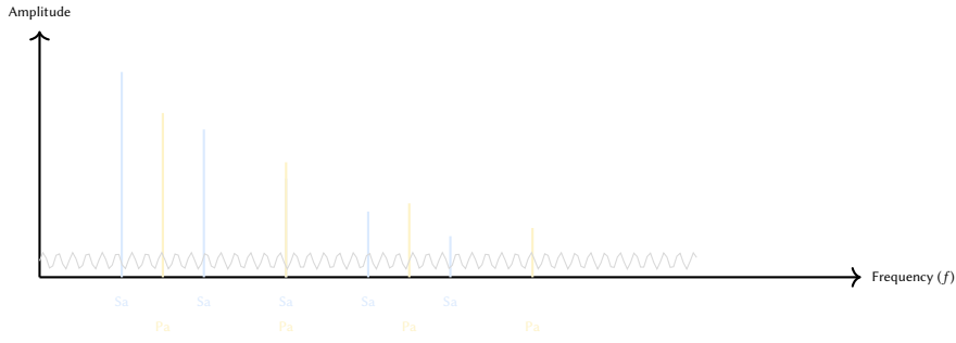
Figure 52. Harmonic spectrum of the Tanpura drone. The fundamental pitches (typically Sa and Pa) are accompanied by a dense series of upper partials that create a continuous, shimmering "bed" of sound. Overtone mimics this via multi-oscillator FM synthesis with slow phase modulations.
