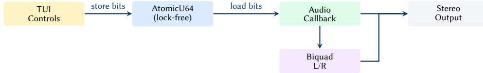
Figure 64. Lock-free live parameter path: the TUI stores f64 bit patterns into atomics; the audio callback loads them each block and updates the biquad filter only when thresholds are exceeded.
