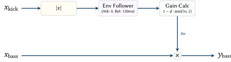
Figure 19. Sidechain compression signal flow. The absolute value of the kick signal drives an envelope follower with instantaneous attack and exponential release. This envelope calculates a dynamic gain reduction ( g_{sc} ) which is multiplied against the bass signal, ducking it to create rhythmic pumping.
