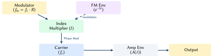
Figure 15. Lead synthesiser signal flow using 2-operator FM.
