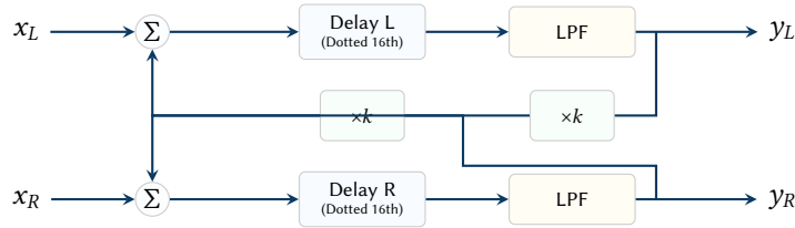
Figure 20. Ping-Pong Delay topology. Left and right channel inputs ( x_L, x_R ) are fed into independent delay lines. The output of each delay line is low-pass filtered (for analog-style damping), multiplied by the feedback coefficient k , and routed into the input sum of the opposite channel's delay line, creating a stereo bouncing effect.
