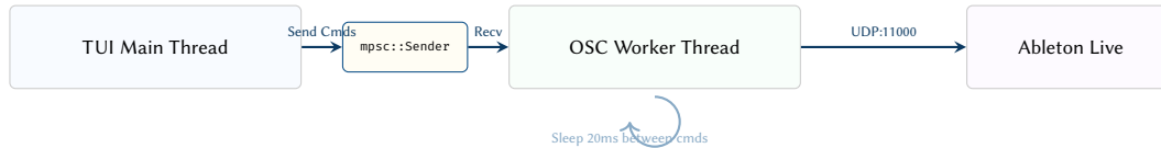
Figure 60. Non-blocking OSC Push architecture. The TUI sends sequences of commands (Delete → Create → Add Notes) via a channel. The background worker consumes this queue and handles the necessary network sleeps without stalling the rendering loop.
