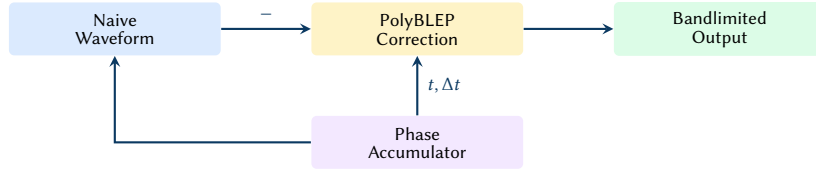
Figure 24. PolyBLEP anti-aliasing: the correction term is subtracted from the naive waveform at phase discontinuities.
