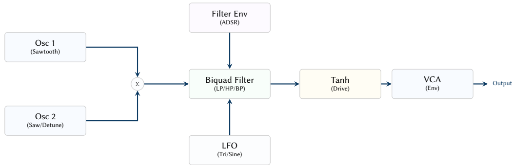
Figure 11. The bass synth signal flow. Dual sawtooth oscillators are summed and passed through a multi-mode biquad filter. Cutoff frequency is modulated by both an ADSR envelope and a free-running LFO. The signal is then saturated via a tanh function and shaped by the VCA envelope.
