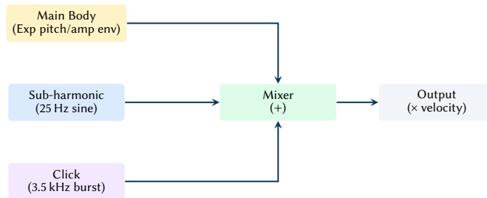
Figure 10. Kick drum synthesis model: parallel summation of main body, sub-harmonic, and click layers.
