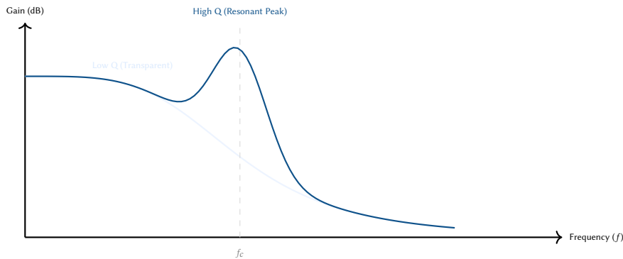
Figure 12. Filter response geometries. The "Acid" character is achieved by a sharp resonant peak at the cutoff frequency ( f_c ). When the cutoff is modulated by a fast envelope, this peak sweeps through the harmonics of the sawtooth oscillator, creating the characteristic "wow" and "squelch" textures.
