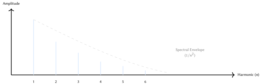
Figure 53. Additive synthesis model for the Shruti Box. The engine sums the first six harmonics of the tonic (Sa) and the fifth (Pa) with amplitudes decaying at a rate of 1/n^2 . A slow bellows-like amplitude LFO is applied to simulate the manual pumping of the instrument.
