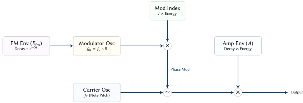
Figure 14. Two-operator FM Synthesis architecture. The modulator oscillator frequency ( f_m ) is a ratio ( R ) of the carrier pitch. The modulation depth (Index I ) is dynamically scaled by the macro energy level, meaning higher energy sections produce much brighter, richer sideband harmonics. The FM envelope ( E_{fm} ) creates a "pluck" or "wow" transient.
