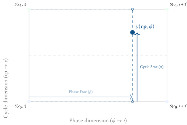
Figure 22. Bilinear cross-cycle interpolation in the Wavetable Oscillator. To prevent zipper noise when sweeping wavetables and aliasing when playing high pitches, the engine first interpolates horizontally between adjacent samples ( i and i + 1 ) within two adjacent wave cycles ( c_0 and c_1 ), and then interpolates vertically between the resulting values.
