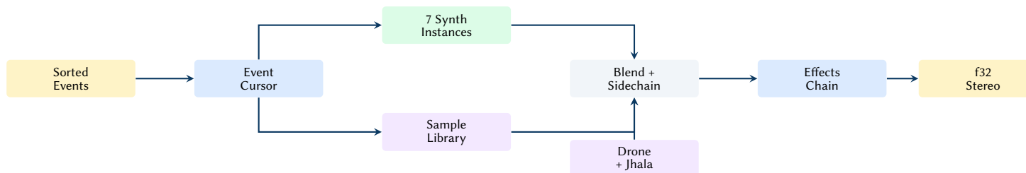
Figure 63. Streaming engine architecture: pre-sorted events are dispatched sample-accurately, blended with energy-aware sample playback, and processed through the effects chain.
