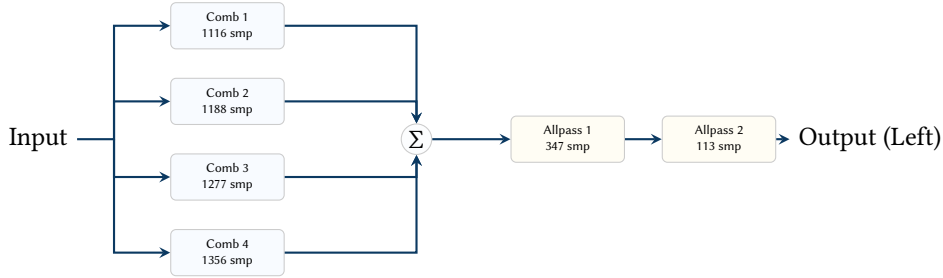
Figure 21. Schroeder Reverb topology (Left Channel). The input signal is fed in parallel to four comb filters with mutually prime delay lengths. Their outputs are summed and passed serially through two allpass filters to increase echo density without coloring the sound.
