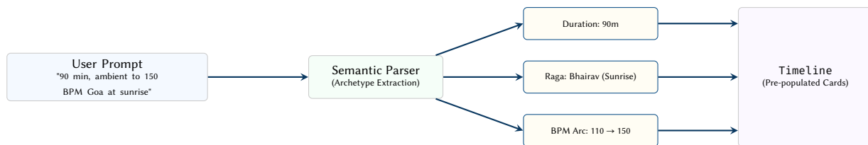
Figure 70. The Oracle Prompt workflow. Natural language is parsed into structural parameters (duration, raga mapping, tempo curves) to algorithmically pre-populate the timeline with thematic cards.
