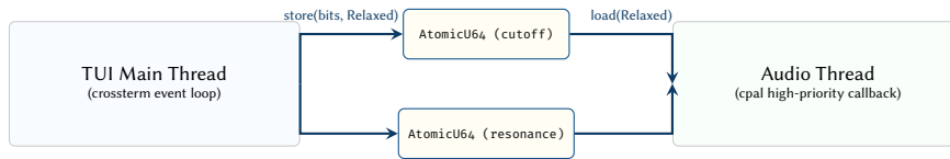
Figure 66. Lock-free concurrency model. The UI thread communicates with the real-time audio thread strictly through atomic variables, preventing priority inversion and guaranteeing that the audio callback never blocks waiting for a mutex.
