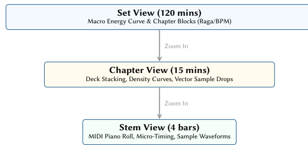
Figure 69. The Semantic Zoom interface. At the macro level, users arrange the global energetic flow. At the micro level, they edit precise MIDI syncopation. Edits made at the stem level automatically recalculate the structural tension displayed at the set level.
