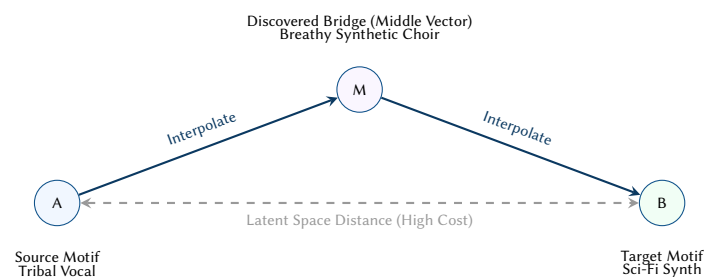
Figure 59. Latent space motif interpolation. When bridging two structurally distant chapters, the engine calculates the latent vector between their respective samples (A and B). It queries the database for a sample (M) that sits mathematically between them, creating a sonically logical bridge that a human might never have searched for.
