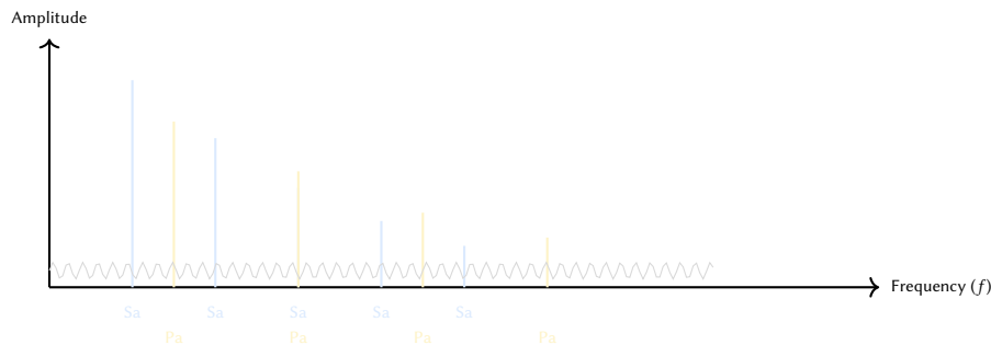
Figure 41. Harmonic spectrum of the Tanpura drone. The fundamental pitches (typically Sa and Pa) are accompanied by a dense series of upper partials that create a continuous, shimmering "bed" of sound. Overtone mimics this via multi-oscillator FM synthesis with slow phase modulations.
