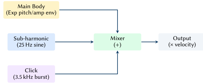
Figure 9. Kick drum synthesis model: parallel summation of main body, sub-harmonic, and click layers.
