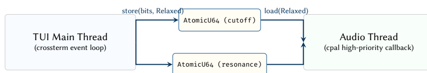
Figure 53. Lock-free concurrency model. The UI thread communicates with the real-time audio thread strictly through atomic variables, preventing priority inversion and guaranteeing that the audio callback never blocks waiting for a mutex.
