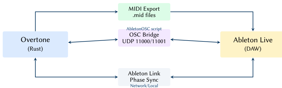
Figure 46. Ableton Live integration architecture. Overtone communicates via Standard MIDI Files for static export, bidirectional OSC for clip pushing and scene control, and Ableton Link for phase-locked transport synchronisation.
