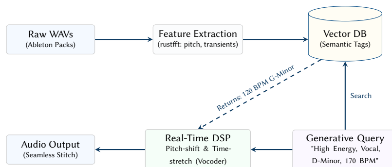
Figure 58. The Semantic Sample Stitching pipeline. During ingestion, samples are analyzed and stored in a vector database. During generation, the engine queries the DB based on the current thematic context, retrieves the best match, and dynamically time-stretches and pitch-shifts the audio to fit the active pocket.
