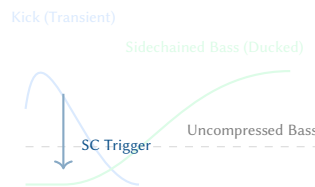
Figure 2. Phase-coherent sidechain alignment. To prevent frequency masking in the critical 40–100 Hz region, Overtone's sidechain compressor attenuates the bass signal during the first 10–20 ms of each kick hit, creating the "pumping" sensation foundational to the genre.
