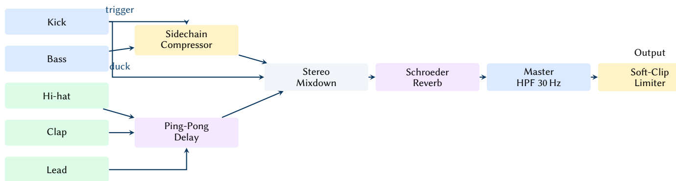
Figure 14. Master effects signal flow. The kick triggers the sidechain compressor which ducks the bass. Hi-hat, clap, and lead pass through the ping-pong delay before joining the stereo bus.
