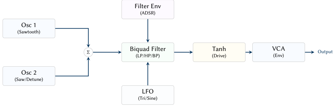
Figure 10. The bass synth signal flow. Dual sawtooth oscillators are summed and passed through a multi-mode biquad filter. Cutoff frequency is modulated by both an ADSR envelope and a free-running LFO. The signal is then saturated via a tanh function and shaped by the VCA envelope.
