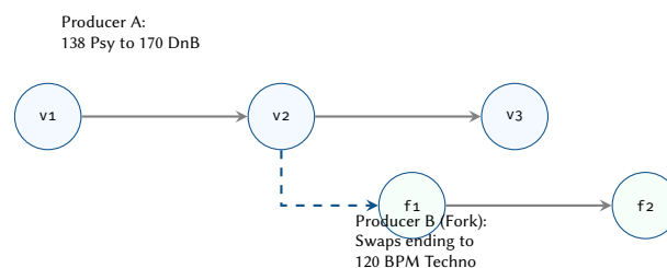
Figure 55. The Generative Git-Tree. Sets can be forked and collaboratively edited. When Producer B swaps the ending chapter, the engine automatically recalculates the transition bridges without requiring the transfer of massive audio stems.
