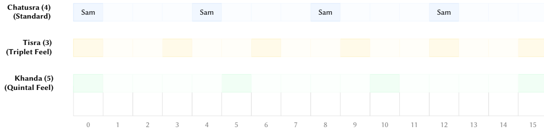
Figure 32. Nadai subdivision masks. By applying these velocity multipliers, Overtone creates the sensation of different pulse groupings (3, 4, 5) while maintaining a strict 4/4 temporal grid. This is used to drive "Eastern Swing" and polyrhythmic lead variations.
