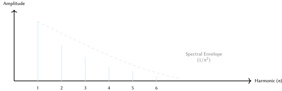
Figure 42. Additive synthesis model for the Shruti Box. The engine sums the first six harmonics of the tonic (Sa) and the fifth (Pa) with amplitudes decaying at a rate of 1/n^2 . A slow bellows-like amplitude LFO is applied to simulate the manual pumping of the instrument.
