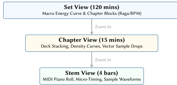
Figure 56. The Semantic Zoom interface. At the macro level, users arrange the global energetic flow. At the micro level, they edit precise MIDI syncopation. Edits made at the stem level automatically recalculate the structural tension displayed at the set level.
