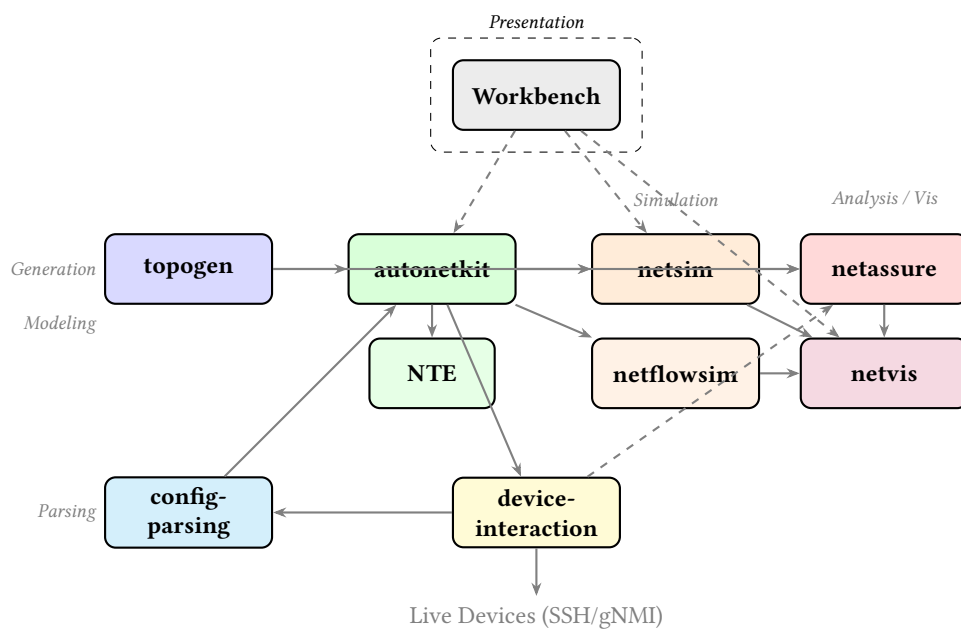
Figure 5: Ecosystem overview: ten tools in architectural layers with data flow arrows. Solid arrows are implemented; dashed arrows are planned.
