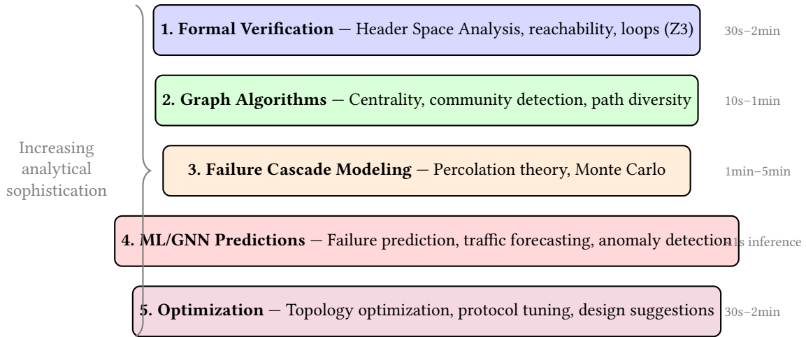
Figure 3: The five analysis paradigms of netassure, with typical compute times.
