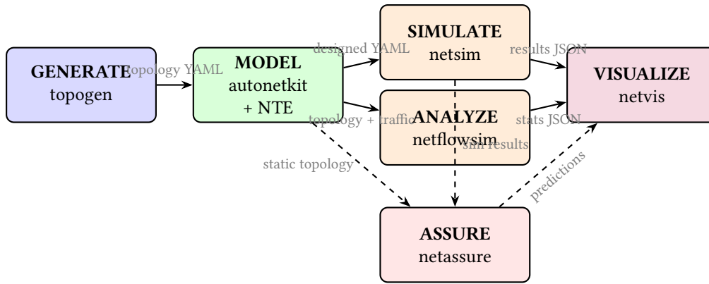
Figure 2: Data flow pipeline. Solid arrows are implemented; dashed arrows are planned or partially implemented.
