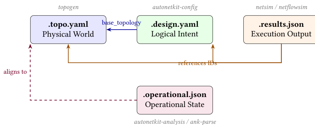
Figure 1: Sidecar file relationships. Solid arrows indicate direct references; dashed arrows indicate identity alignment.
