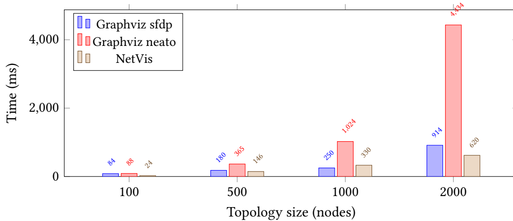
Figure 5: Comparative performance on identical spine-leaf topologies. NetVis includes the full pipeline (layout, labels, styling, SVG render); Graphviz includes layout and SVG output only. Apple M4 Pro, 24 GB RAM, best of 3 runs.
