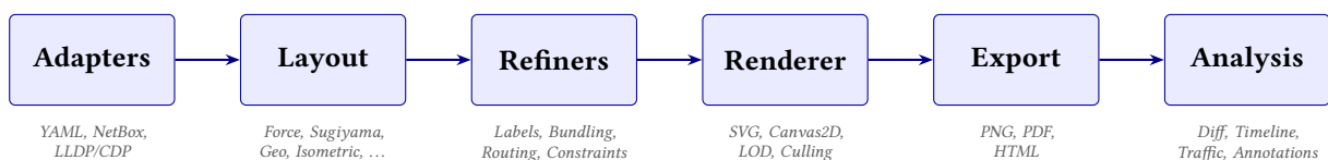
Figure 4: The NetVis six-layer pipeline.
