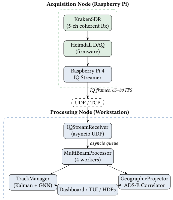
Figure 1: System topology. The acquisition node handles only IQ capture and streaming; all signal processing runs on the workstation.
