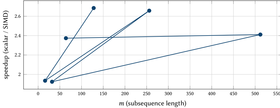
Figure 20. SIMD speedup for centered sumproducts initialisation (Criterion). Generated by make -C docs/report bench-report .
