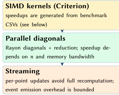
Figure 19. Observed performance effects (representative). SIMD acceleration yields large constant-factor wins in the hot inner kernels; parallel diagonal processing provides further throughput gains when memory bandwidth permits.
