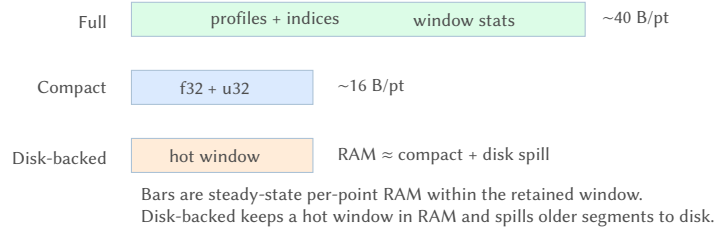
Figure 24. Memory overhead by mode (conceptual). Compact mode reduces per-point storage by narrowing statistics and profile representations; disk-backed mode caps RAM by spilling segments to persistent storage.
