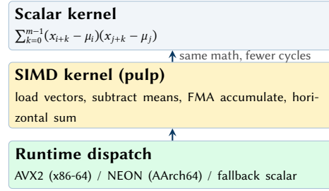
Figure 6. SIMD acceleration strategy. pulp [7] selects an optimal vectorised implementation at runtime while preserving a scalar fallback path.
