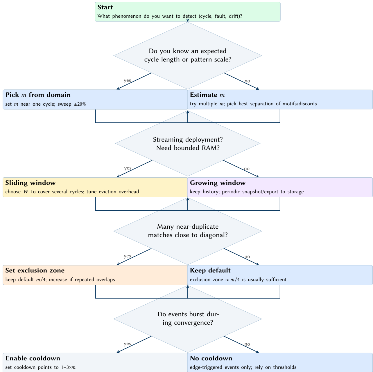
Figure 25. Parameter selection flowchart. Start from domain time scales for m , pick a memory mode (sliding vs growing), keep a conservative exclusion zone, and add cooldown when event streams become noisy.
