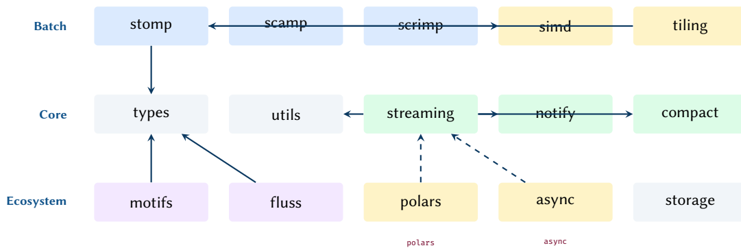
Figure 5. Module architecture. Batch algorithms (top) share SIMD kernels and core types. The streaming engine (middle) builds on the same utilities. Ecosystem integrations (bottom, dashed) are gated behind optional feature flags.
