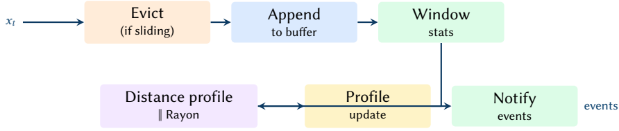
Figure 11. Data flow through append_point . Eviction (orange) only executes in sliding mode. The distance profile computation is parallelised across windows via Rayon.
