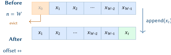
Figure 12. Sliding window eviction. When the buffer is full ( n = W ), the oldest point x_0 is evicted before x_t is appended. The global offset increments to maintain absolute indexing.
