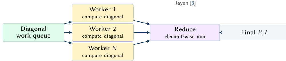
Figure 7. Parallelisation over diagonals. Each diagonal is processed independently on a Rayon worker thread; partial results are merged with an element-wise minimum reduction.
