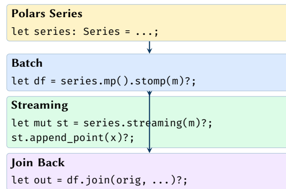
Figure 14. DataFrame-native workflow. A Polars Series produces a batch profile as a DataFrame, can transition to streaming, and can be joined back into wider feature pipelines.
