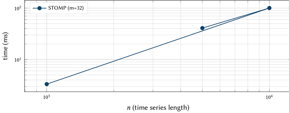
Figure 17. End-to-end STOMP scaling (Criterion, representative). Log-log axes emphasise the rapid growth in compute cost with n for exact batch joins. Values match Table 3.
