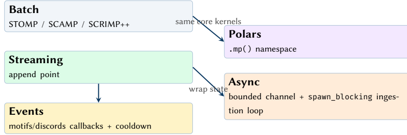
Figure 4. API at a glance. matrix-profile-rs exposes batch, streaming, and ecosystem integration entrypoints that share the same core kernels and profile representations.
