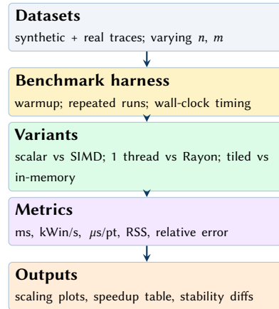
Figure 22. Evaluation methodology flow. We run controlled benchmark variants and report both throughput and correctness metrics to avoid performance-only optimisation bias.
