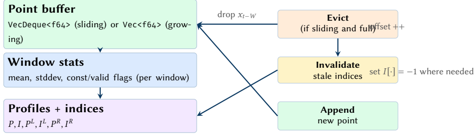
Figure 9. Streaming state layout and sliding-window bookkeeping. In sliding mode, eviction shifts the global offset and requires index invalidation for any neighbour references that now fall outside the retained window.
