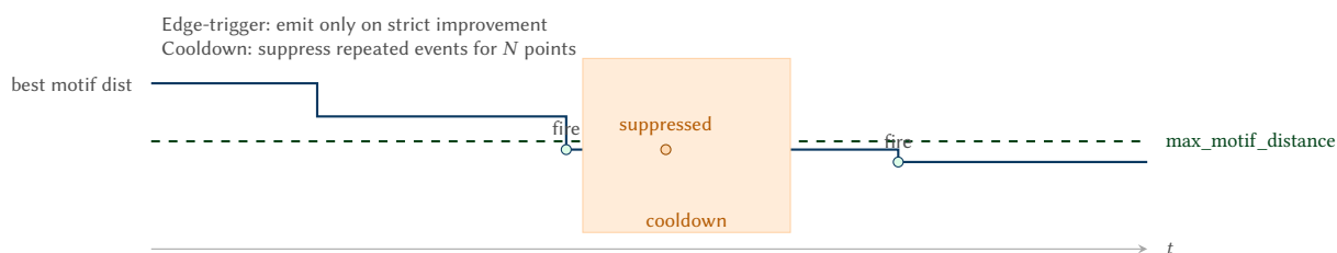
Figure 13. Notification semantics (motifs shown). Events are edge-triggered: a motif event fires only when the global best-so-far distance strictly improves past the configured threshold. A cooldown window suppresses repeated events during rapid convergence.
