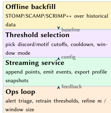
Figure 16. Operational use case loop. A common pattern is to backfill exact profiles offline, derive thresholds, then run a long-lived streaming service with periodic recalibration.
