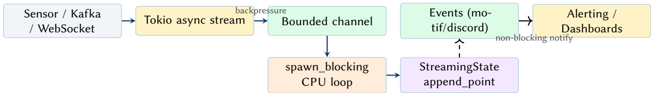
Figure 15. Async deployment pattern. An async source feeds a bounded channel; CPU-bound updates run on spawn_blocking , while event notifications are delivered without stalling ingestion.
