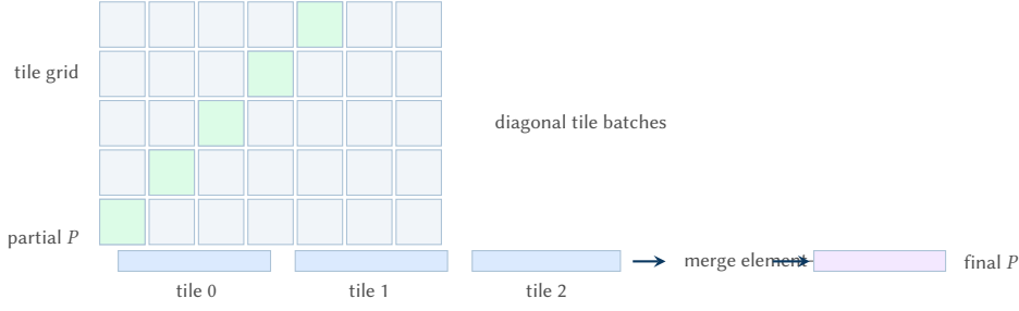
Figure 8. Tiled STOMP for out-of-core datasets. stomp_tiled processes the distance matrix in memory-bounded tiles, producing partial profiles that are merged via an element-wise minimum reduction to yield the final Matrix Profile.
