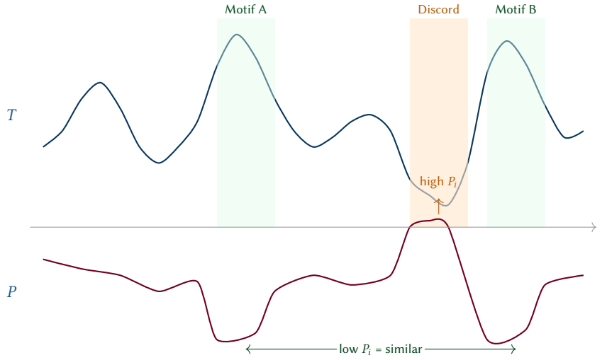
Figure 2. Conceptual overview. A time series T (top) contains a repeated motif (green) and an anomaly (orange). The Matrix Profile P (bottom, purple) assigns low distances to motif positions and high distances to the discord. Reading the profile’s minima yields motifs; its maxima yield discords.
