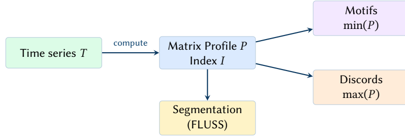
Figure 3. Matrix Profile downstream tasks. The profile vector P supports motif and discord discovery via extrema, while the index vector I supports regime change detection via FLUSS [6].
