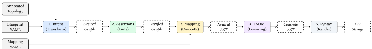
Figure 14. NetCfg compilation pipeline. High-level intent is progressively lowered through three distinct AST representations (Verified Graph, Neutral AST, Concrete AST) before serialisation.
