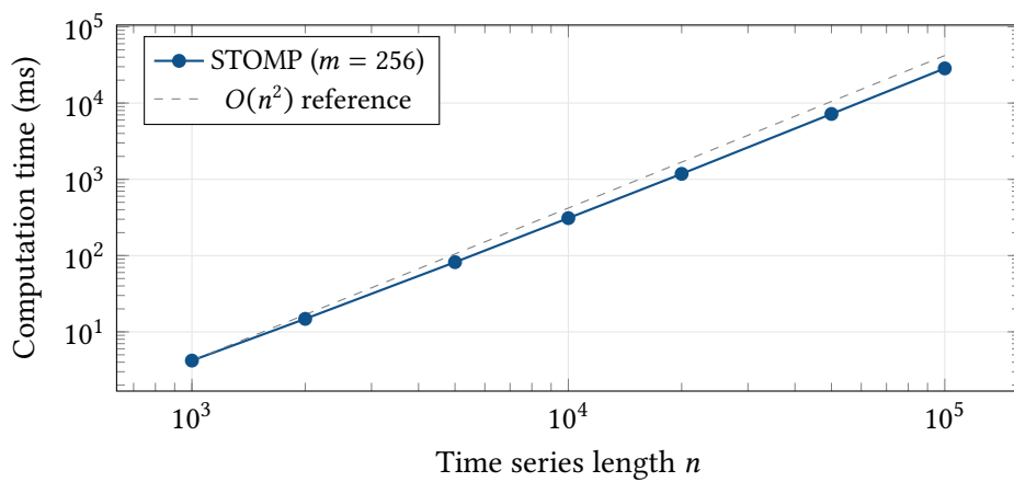
Figure 22. STOMP batch scaling. Measured times track ideal O(n^2) scaling closely across two orders of magnitude.
