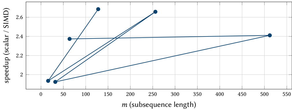
Figure 19. SIMD speedup for centered sumproducts initialisation (Criterion). Generated by make -C docs/report bench-report .
