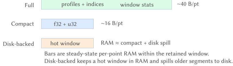
Figure 23. Memory overhead by mode (conceptual). Compact mode reduces per-point storage by narrowing statistics and profile representations; disk-backed mode caps RAM by spilling segments to persistent storage.
