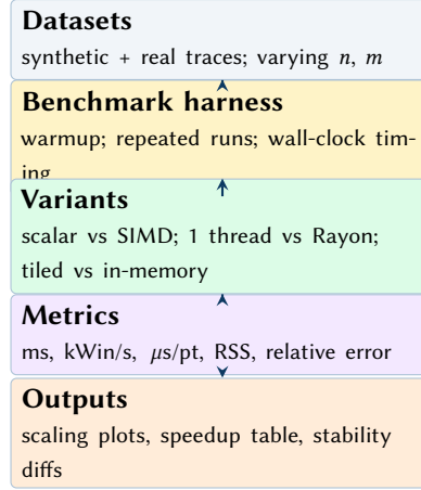
Figure 21. Evaluation methodology flow. We run controlled benchmark variants and report both throughput and correctness metrics to avoid performance-only optimisation bias.
