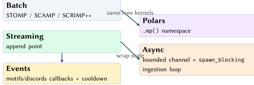
Figure 3. API at a glance. matrix-profile-rs exposes batch, streaming, and ecosystem integration entry-points that share the same core kernels and profile representations.
