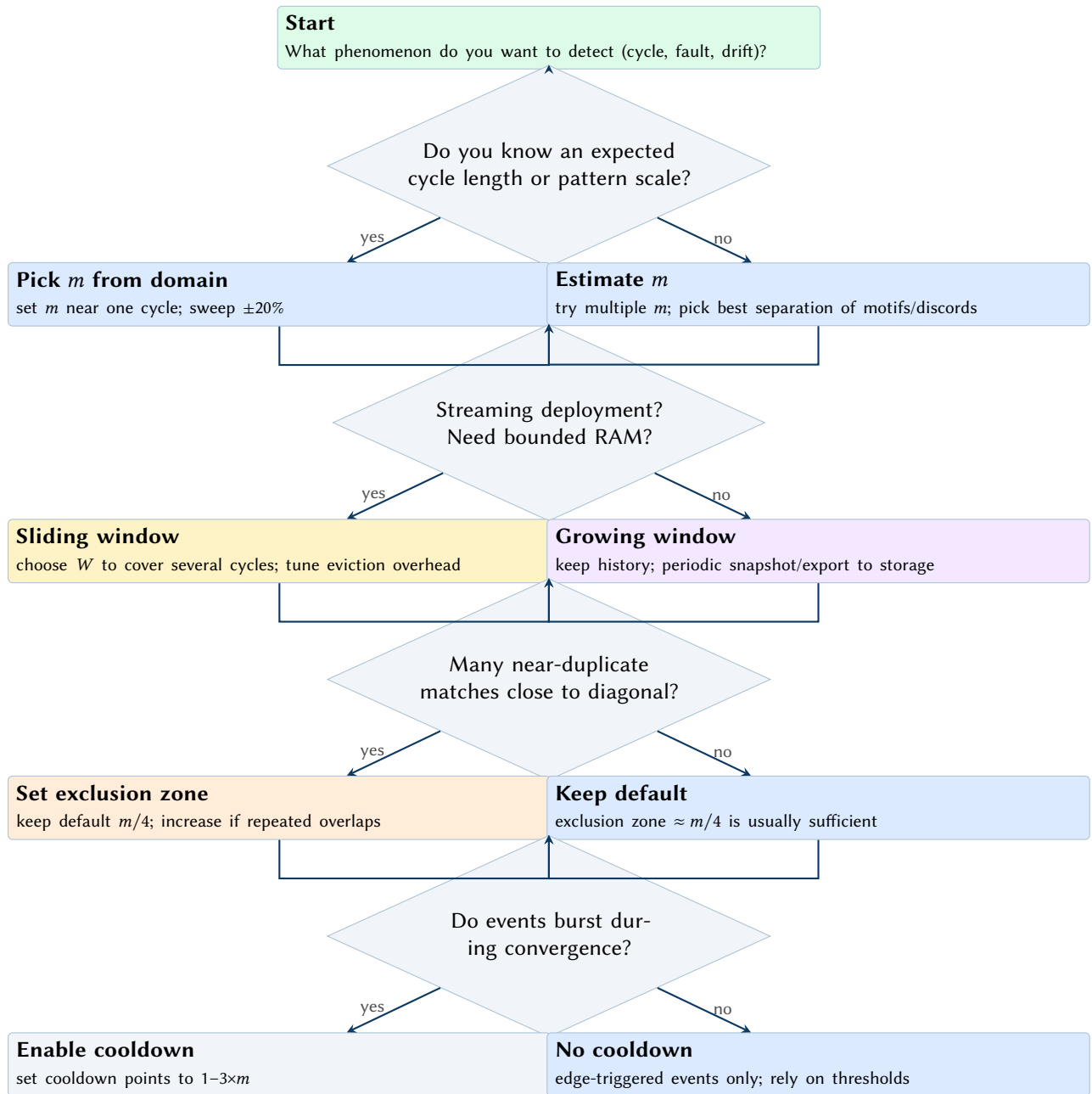
Figure 24. Parameter selection flowchart. Start from domain time scales for m , pick a memory mode (sliding vs growing), keep a conservative exclusion zone, and add cooldown when event streams become noisy.
