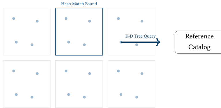
Figure 41. The native plate solver uses quad-hashing (fig. 38) to perform sub-millisecond lookups against a pre-compiled K-D tree of the sky, enabling blind astrometry on devices without internet access or heavy dependencies.
