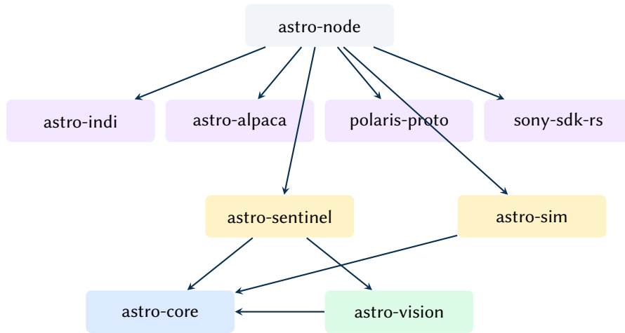
Figure 1. Crate dependency hierarchy. Arrows point from dependant to dependency. The two crates at the base contain all pure computation; upper layers add I/O and device interaction.
