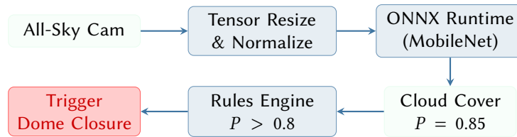
Figure 36. The Sentinel Safety Engine pipeline. Real-time imagery is processed via a cross-platform ONNX inference runtime. The resulting classification probabilities are evaluated against user-defined TOML rules to trigger emergency hardware shutdowns.
