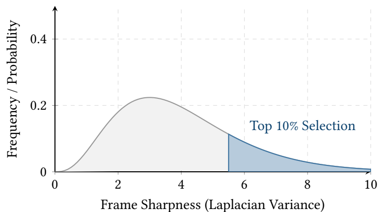
Figure 32. Frame sharpness distribution in a Lucky Imaging sequence. The highly skewed right tail represents the rare frames captured during moments of negligible atmospheric turbulence, which are retained for stacking.
