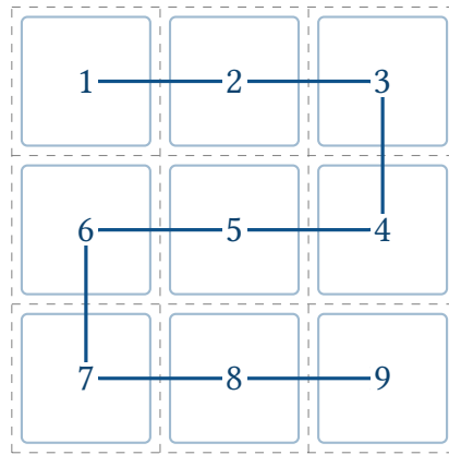
Figure 33. A 3 \times 3 mosaic grid demonstrating the boustrophedon (serpentine) path ordering to minimize mount slew distance.
