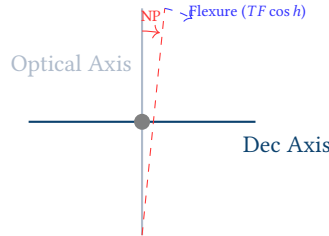
Figure 28. Mount Kinematics. The pointing model corrects for six fundamental mechanical errors: Index errors ( IH, ID ), Polar Elevation/Azimuth ( ME, MA ), Non-perpendicularity ( NP ), and Tube Flexure ( TF ).
