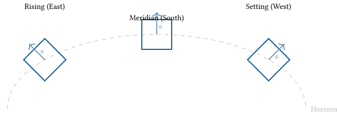
Figure 30. The field rotation effect on an Alt-Az mount. The target (represented by the sensor frame) rotates relative to the celestial field as it traverses the sky, requiring active mechanical derotation for long exposures.
