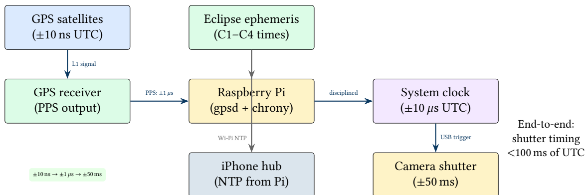
Figure 44. GPS time synchronization hierarchy: satellite signals provide nanosecond-accurate UTC, the GPS receiver’s PPS output disciplines the Raspberry Pi’s system clock via chrony, and USB camera triggers achieve <100 ms end-to-end timing accuracy. The iPhone hub synchronizes via NTP from the Pi nodes.
