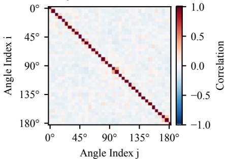
QK Learned Structure
