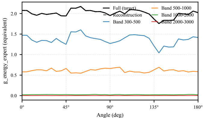
Fig5 B3 Physics band decomposition Sign-aligned decomposition ( \Sigma bands = full)
