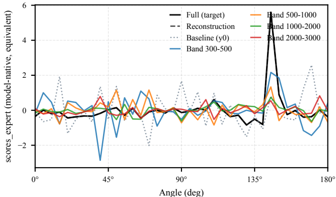
Fig5 B3 QK band decomposition Integrated Gradients attribution (base + \Sigma bands = full)
