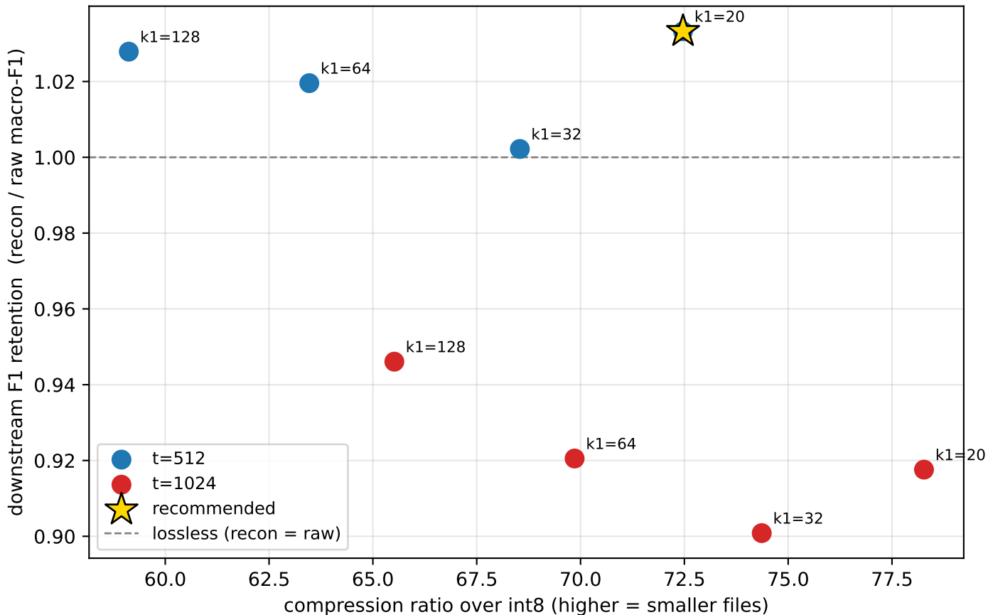
VQ compression vs downstream accuracy — austria (4-fold spatial CV)
