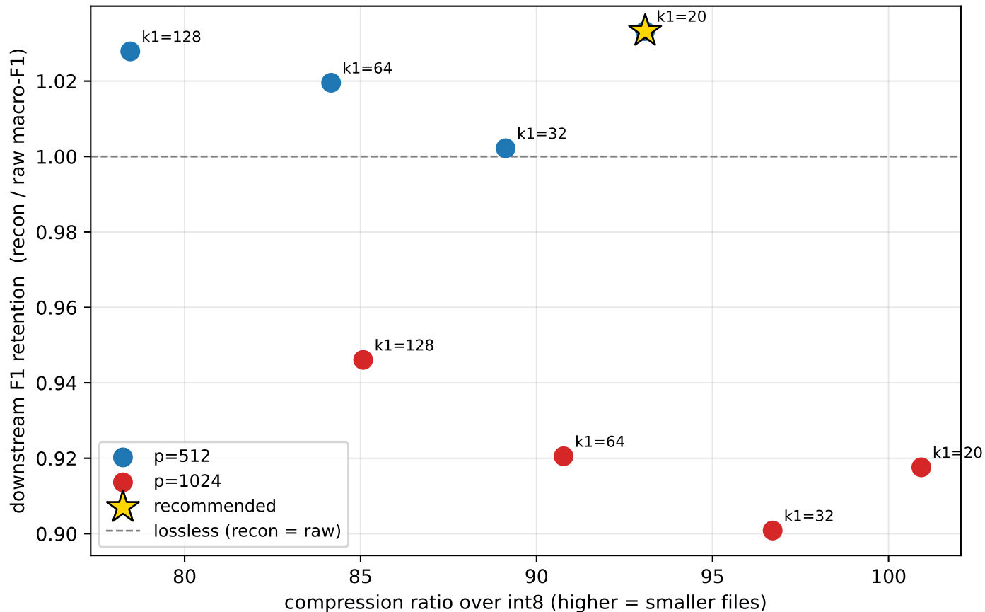
VQ compression vs downstream accuracy — austria (4-fold spatial CV)
