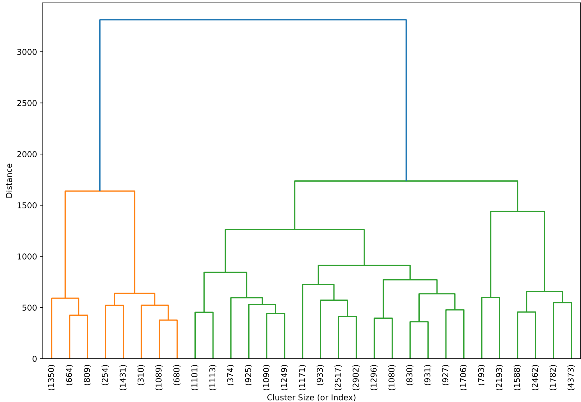
Hierarchical Clustering Dendrogram - All Splits
