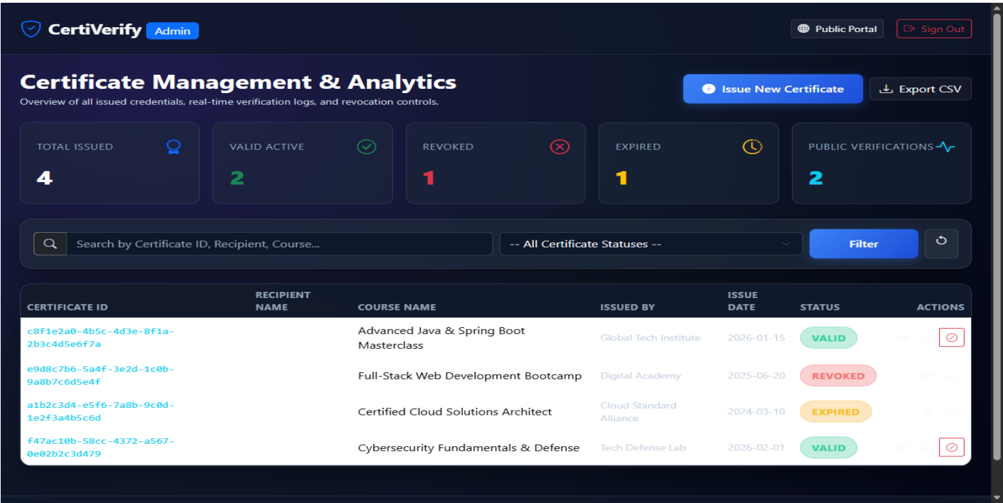
Figure 2.4: Admin Dashboard — System Statistics, Certificate Management Table & CSV Export
