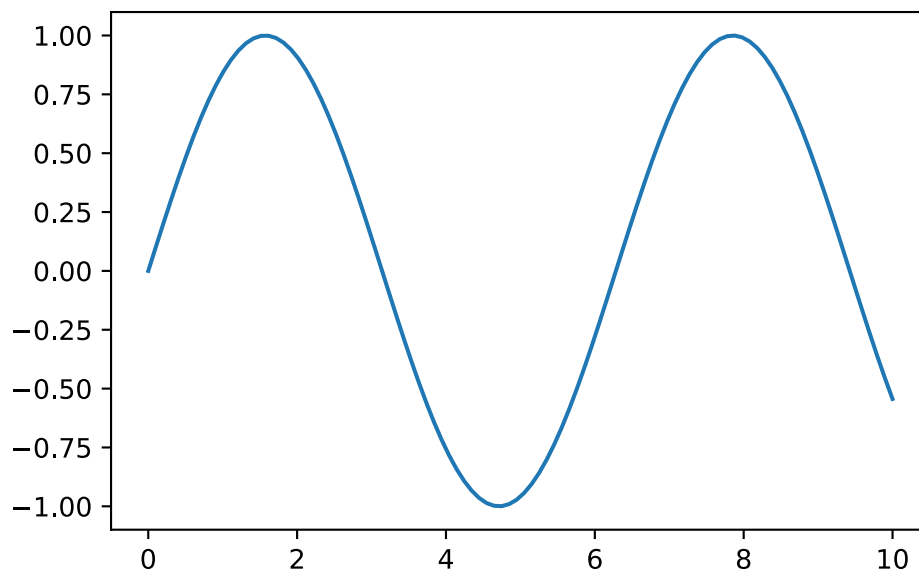
Figure 1: Test Figure
