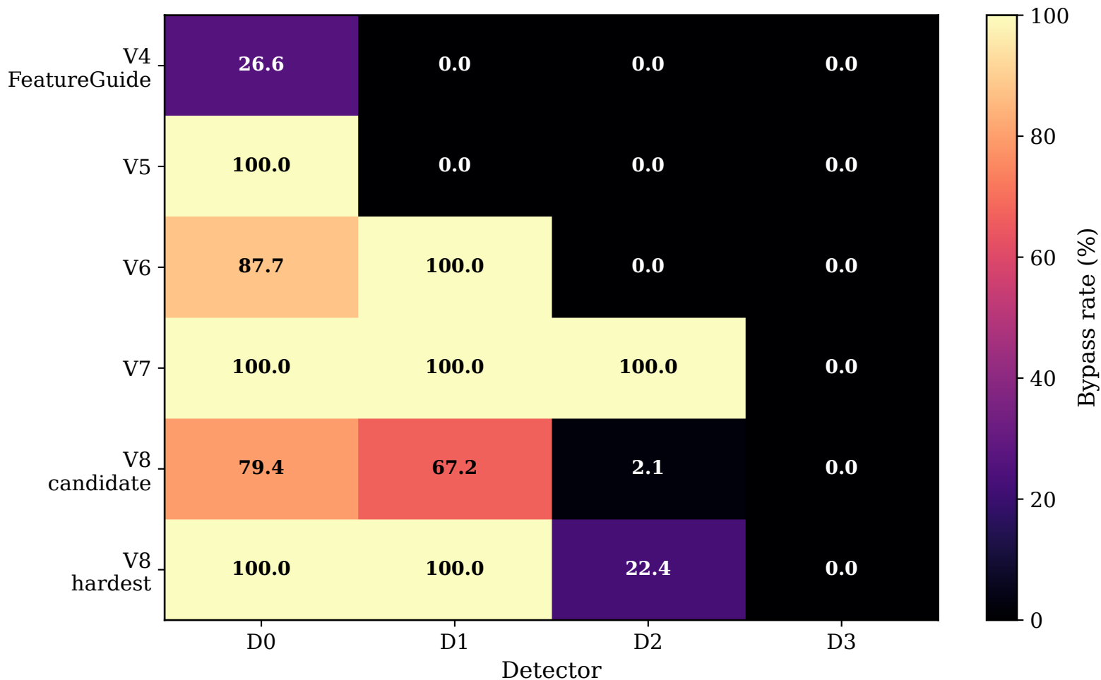
OR90 bypass rate across detectors and adaptive attack rounds
