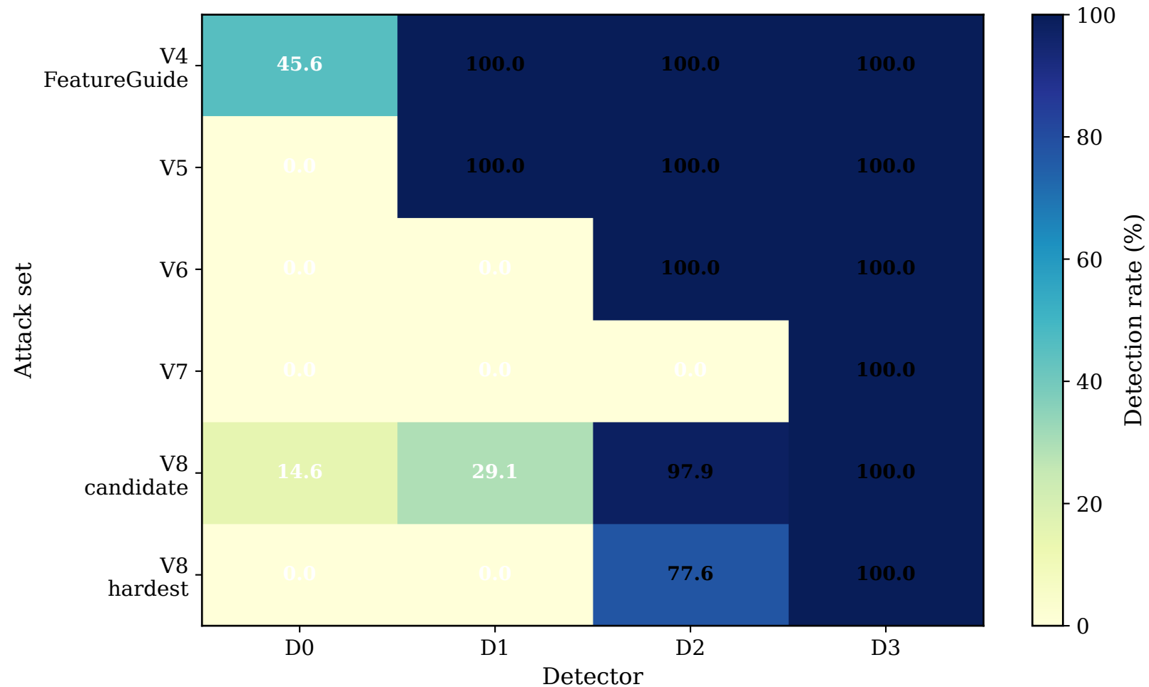
OR95 detection rate across detectors and adaptive attack rounds
