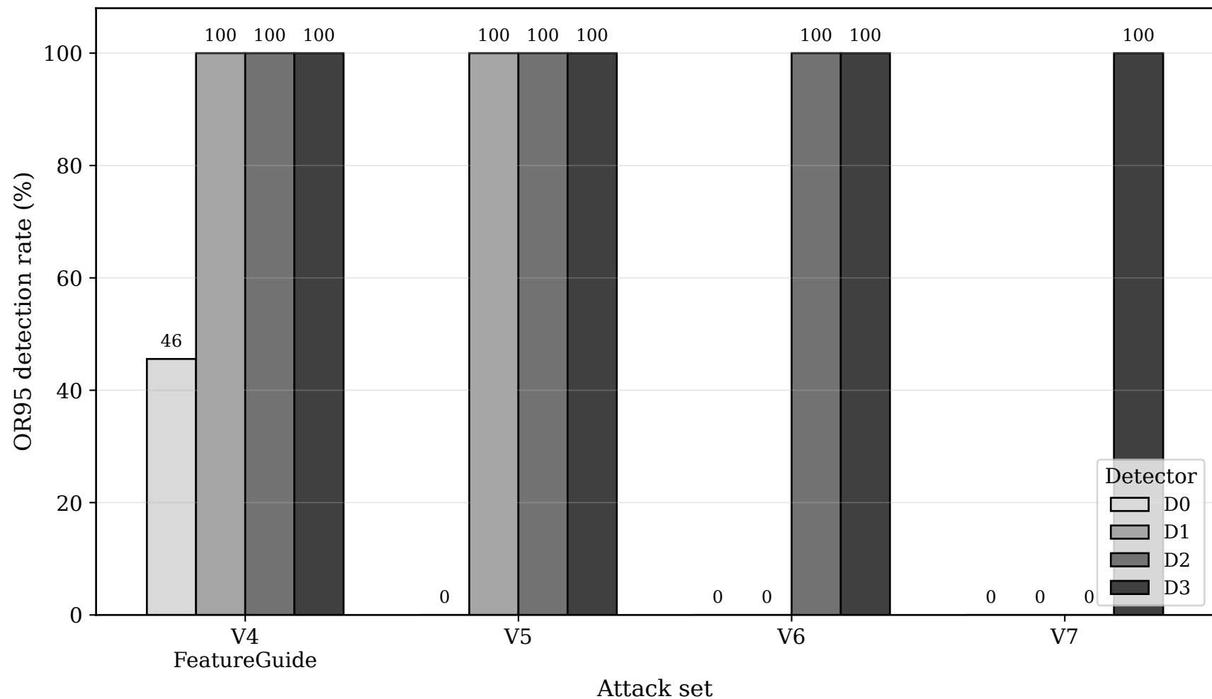
Detector performance progression across adaptive attack rounds
