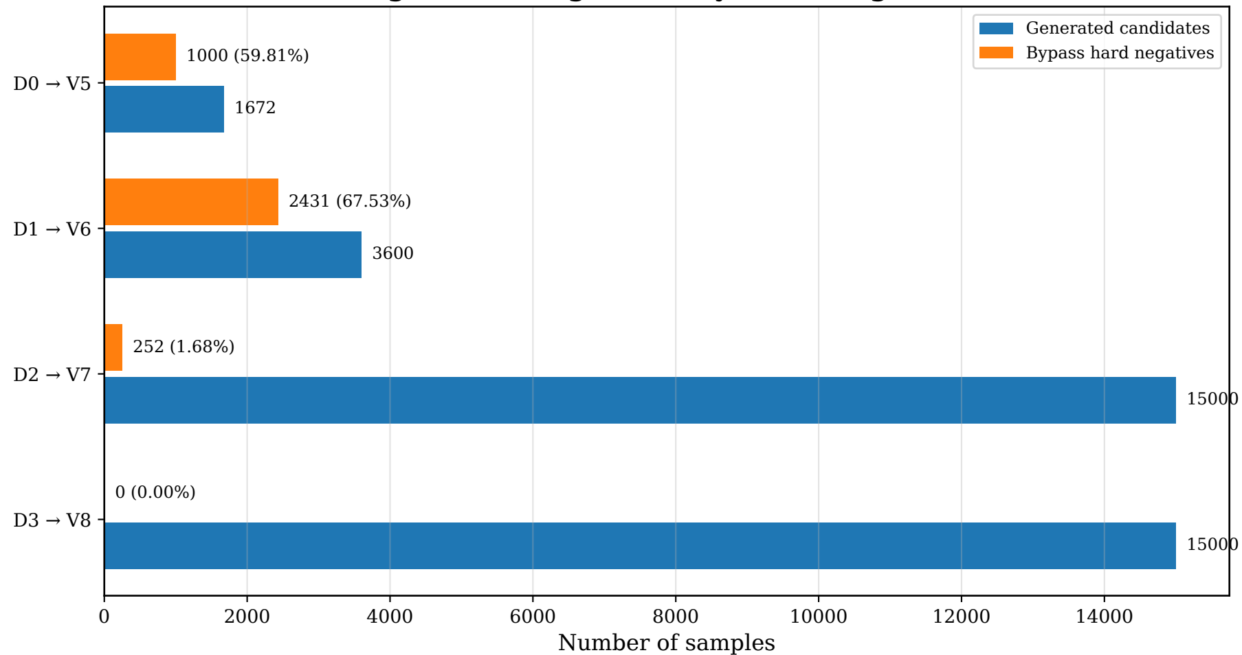
Hard-negative mining funnel by detector-guided round
