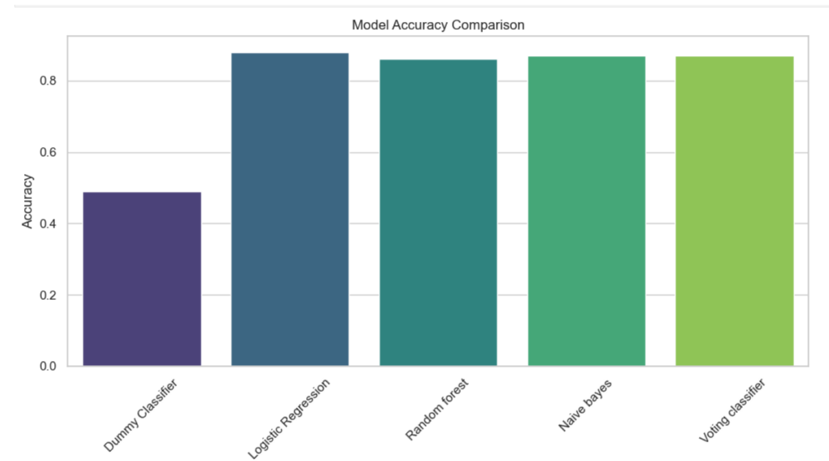
Figure 7: The accuracy of each model
