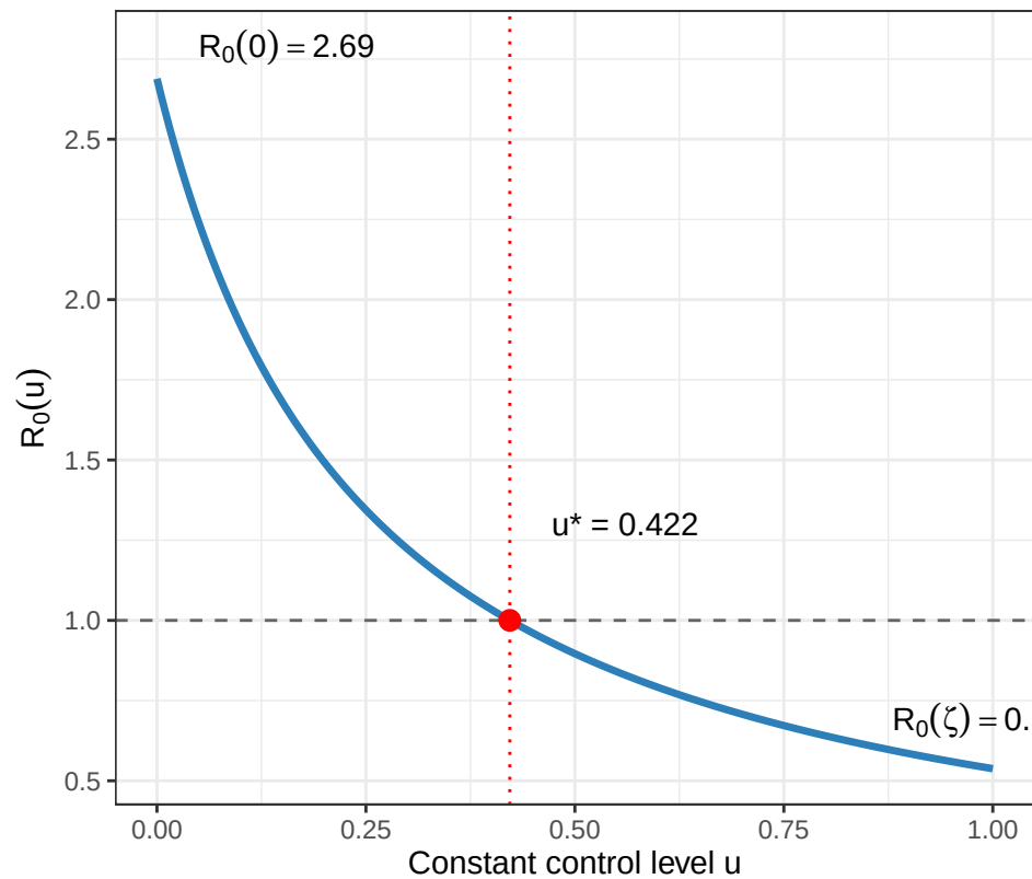
(a) Basic reproduction number
