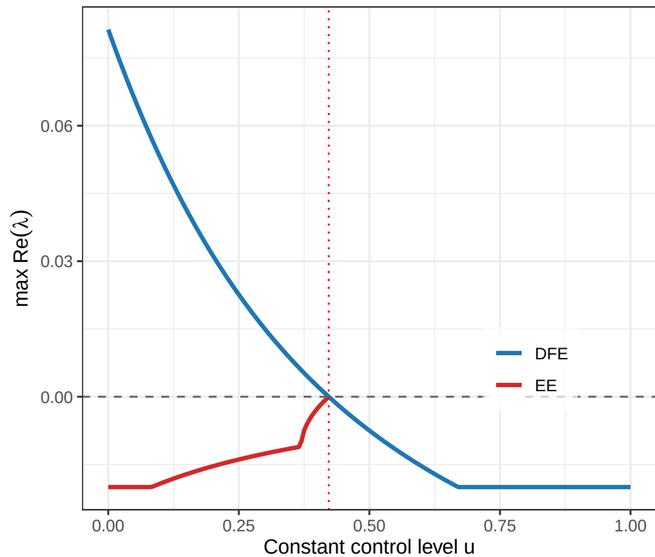
(b) Linear stability: transcritical bifurcation at u^*
