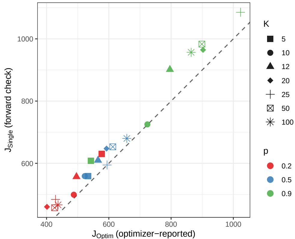
(a) Optimistic bias: 21/21 points above y = x
