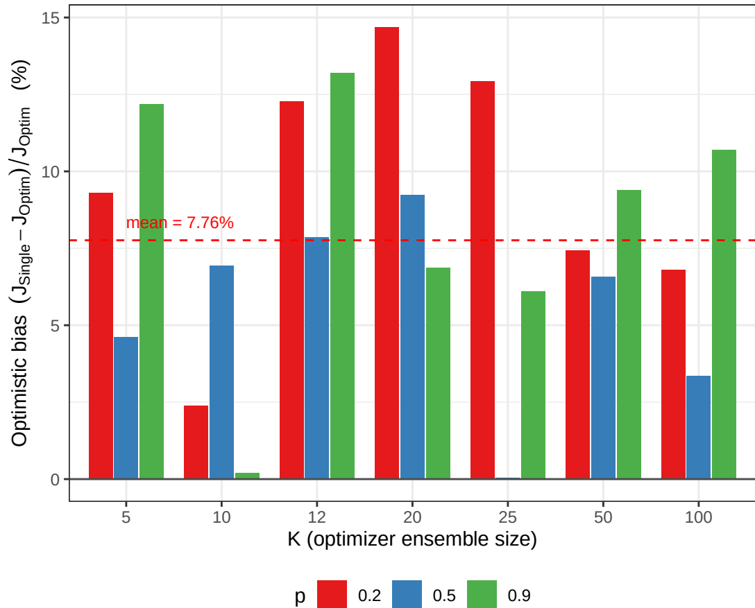
(b) Bias distribution by K and p
