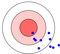
High Bias High Variance
