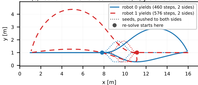
(c) round 2: core names robots 0, 1; yield re-solves
