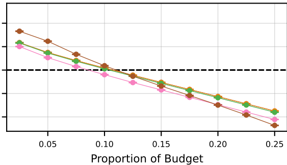
BBH+GPQA+IFEval+MATH+MuSR
