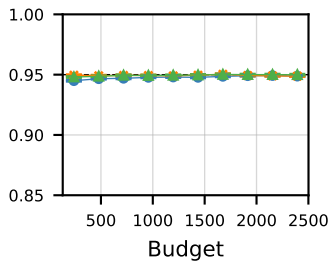
BBH+GPQA+IFEval +MATH+MuSR
