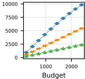
BBH+GPQA+IFEval +MATH+MuSR
