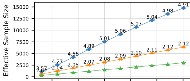
MMLU-Pro
