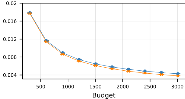
RMSE
