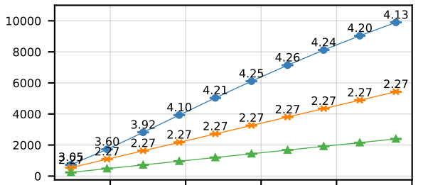
BBH+GPQA+IFEval+MATH+MuSR
