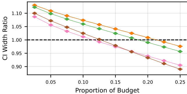
MMLU-Pro
