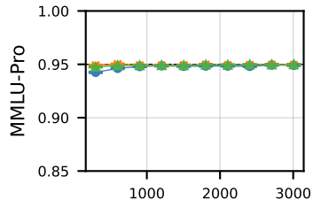
BBH+GPQA+IFEval +MATH+MuSR
