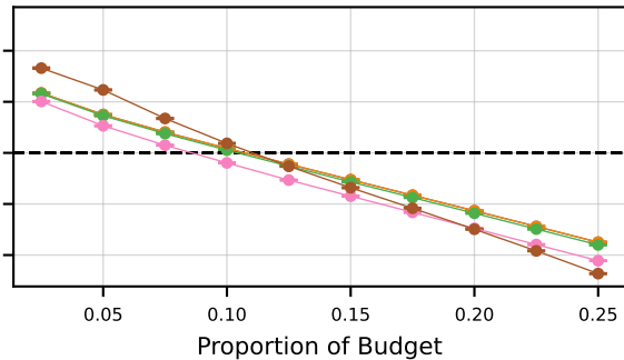
BBH+GPQA+IFEval+MATH+MuSR
