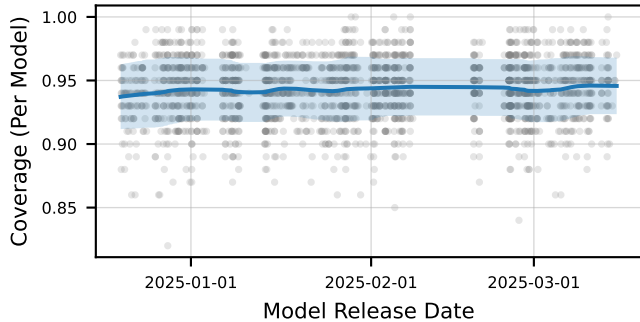
Per-Model Coverage vs. Model Release Date
