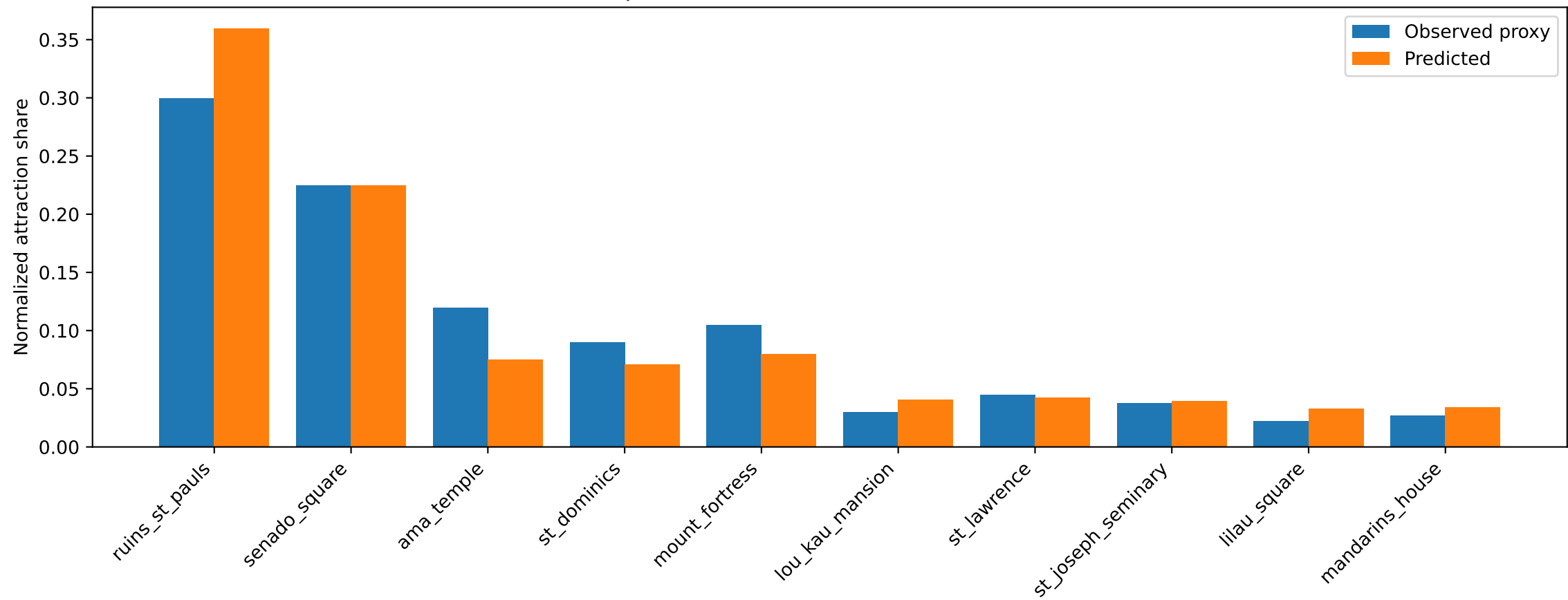
EXP-05 predicted vs observed attraction distribution
