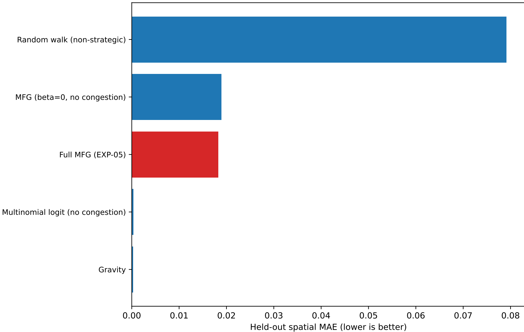
EXP-10: model comparison on the EXP-05 held-out split
